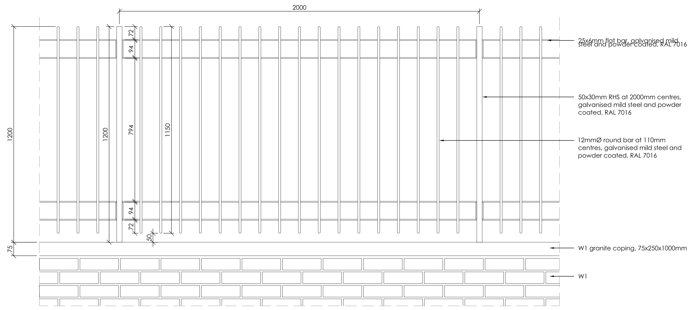
R1 Rolling to Top of Wall Typical Detail Q40/340A 1:10
