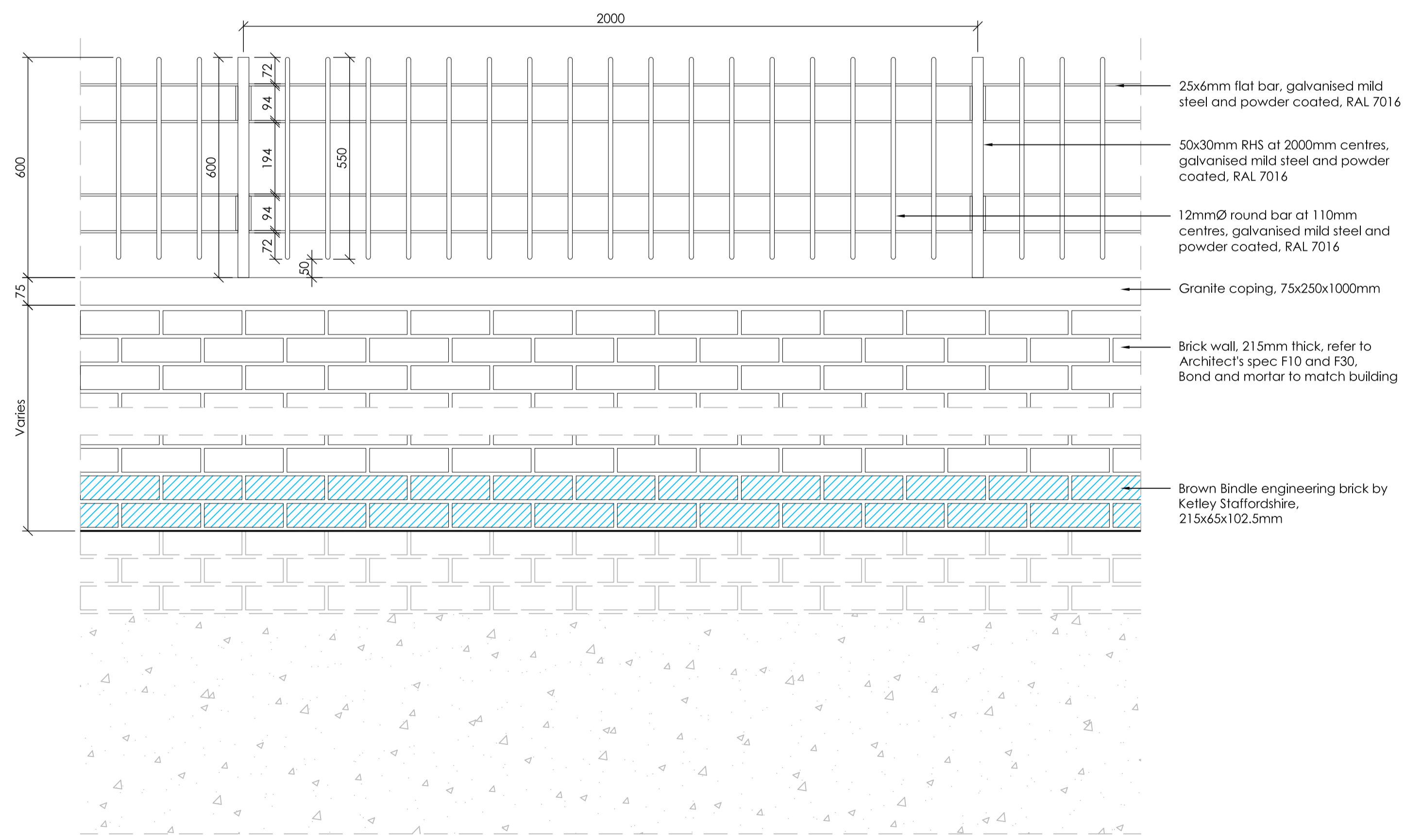
R2 Railing and Wall to Grafton Terrace Typical Detail Q40/340B F10/385A 1:10
