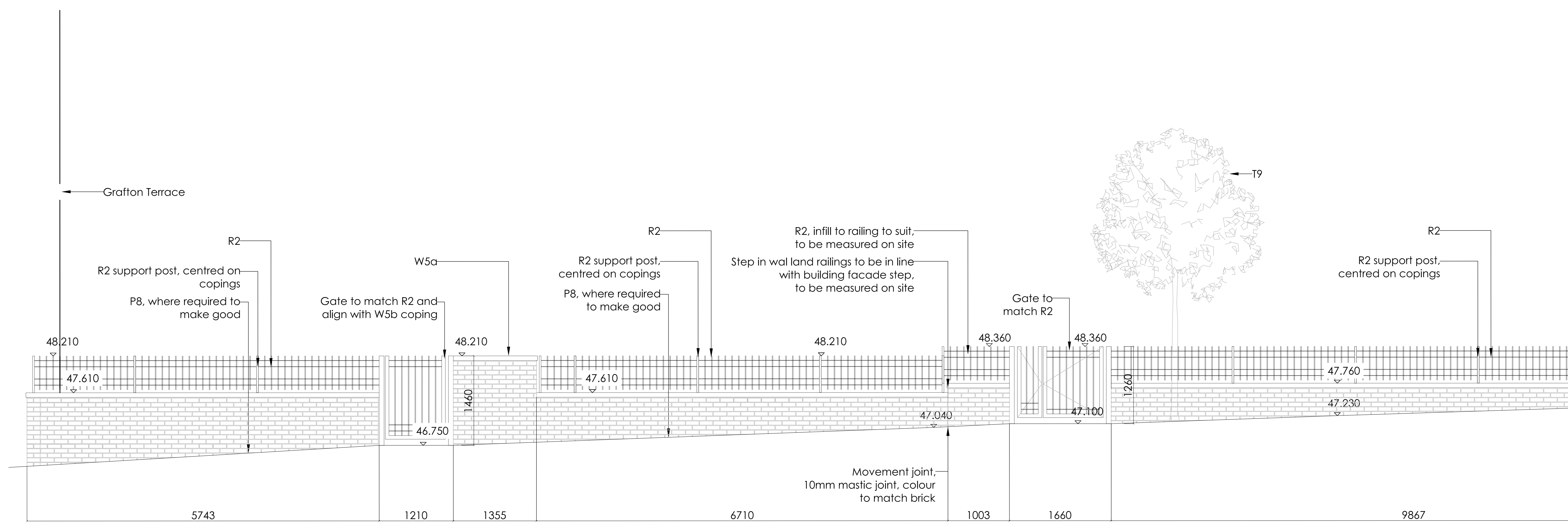
Grafton Terrace Section 1 - Part 1 1:25
