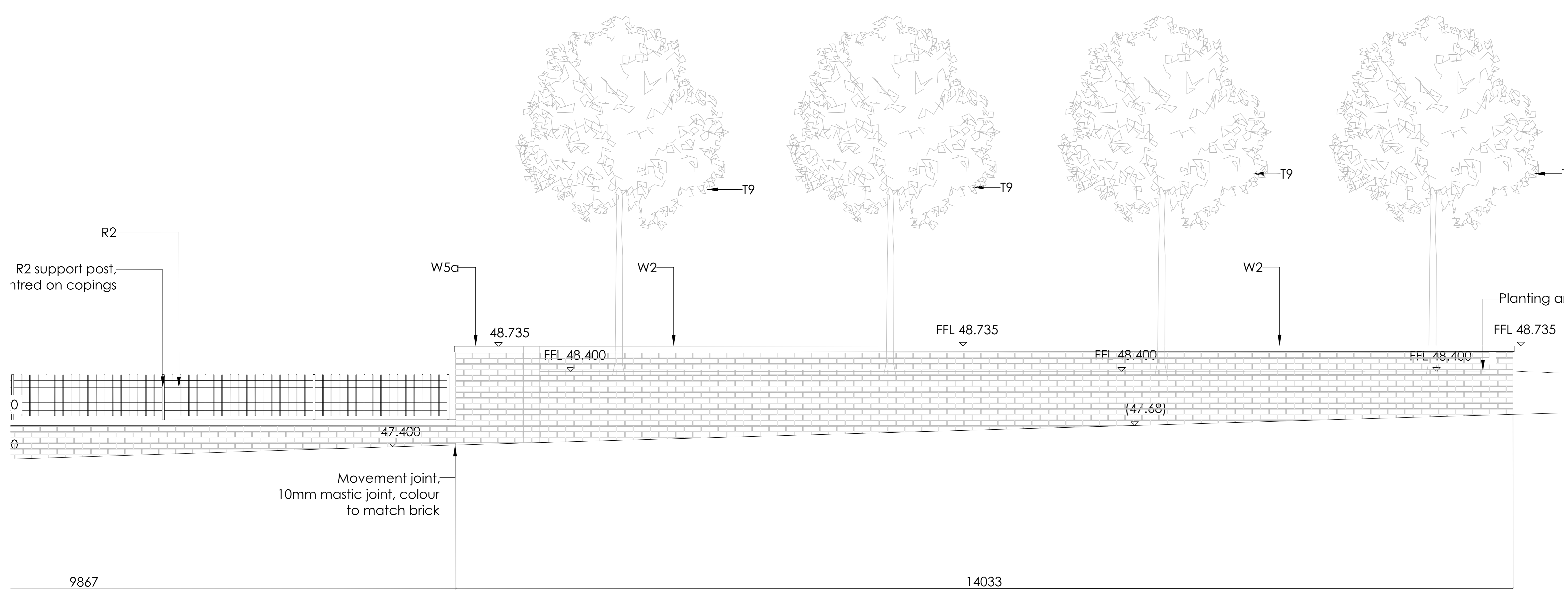
Grafton Terrace Section 1 - Part 2 1:25
