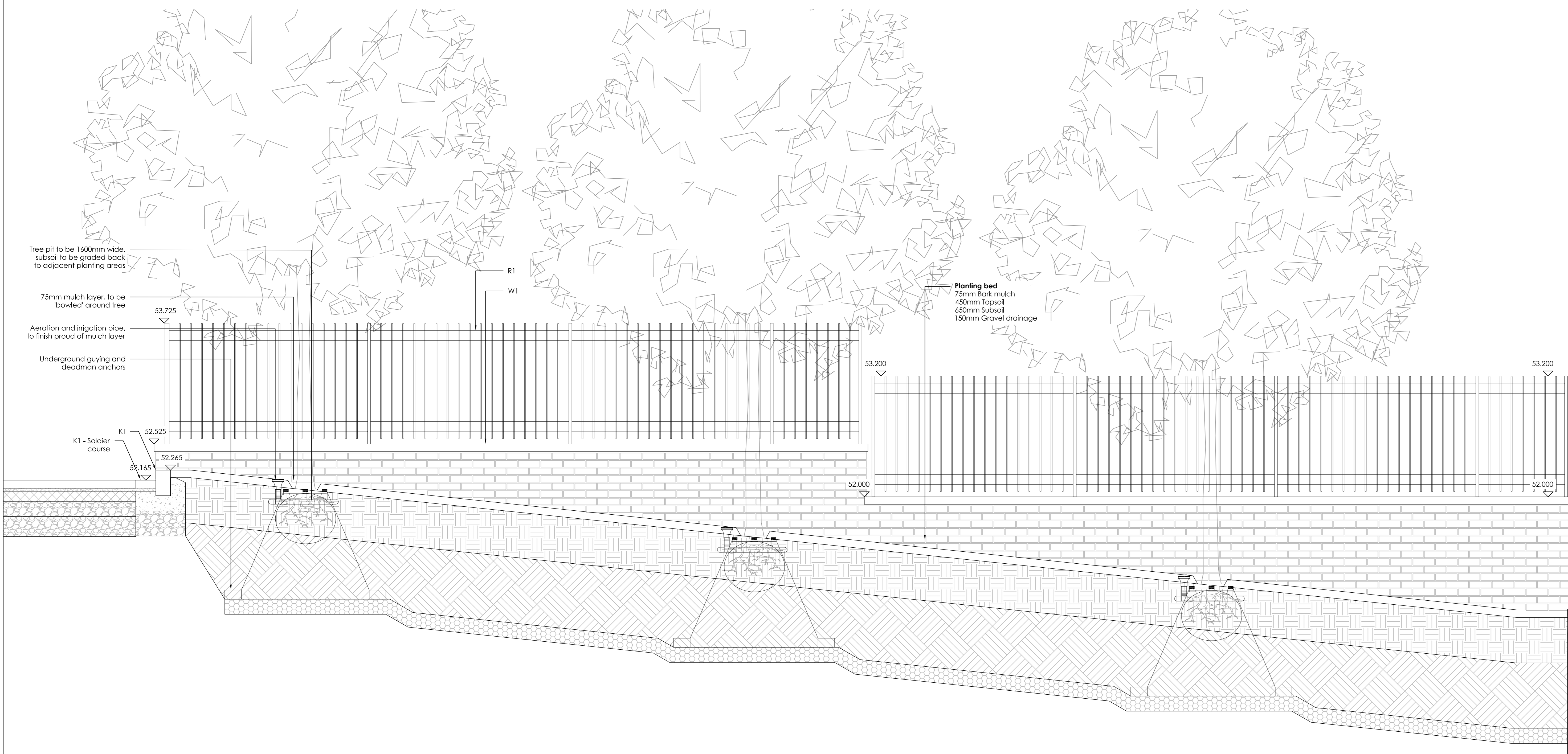
Aspen Villas Southern Boundary Section 1 - Part 2 1:20
