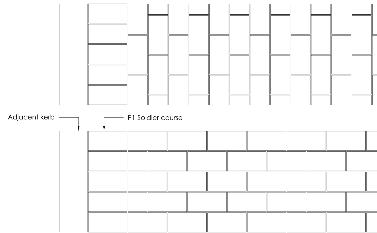
P1 Concrete Block Paving - Bond Detail Q24/115B 1:10
