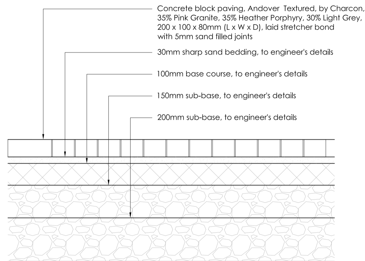
P1 Concrete Block Paving Build-up Detail Q24/115B 1:10
