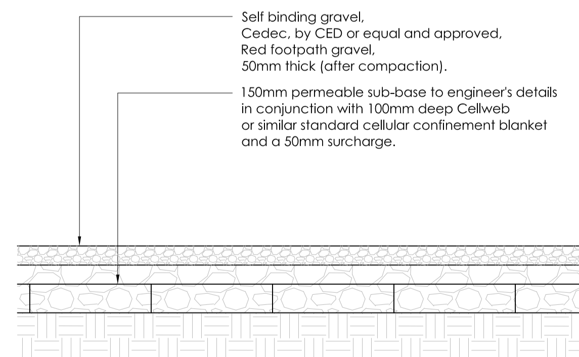
P3a Self Binding Gravel Beneath Existing Trees Build-up Detail Q23/110A 1:10
