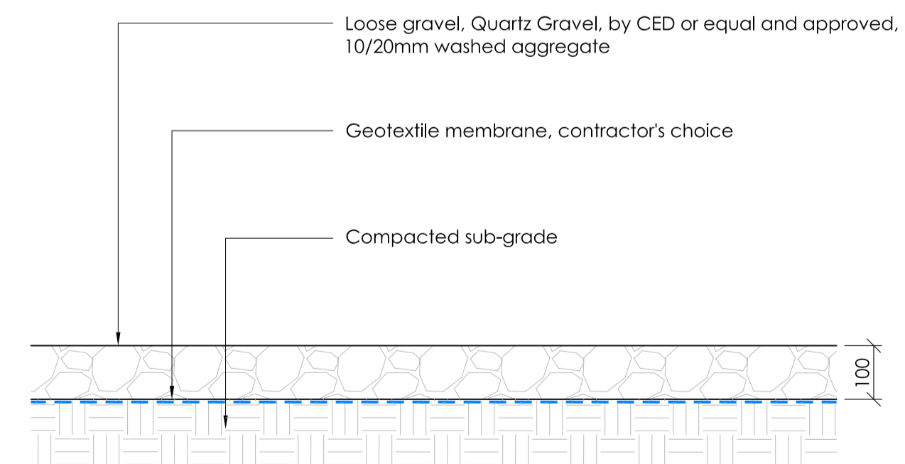
P4 Loose gravel Build-up Detail Q23/160B 1:10
