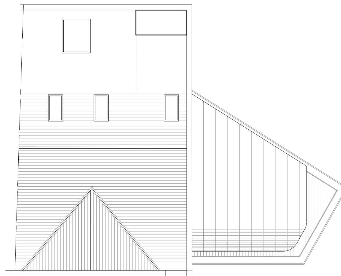
Roof Plan
