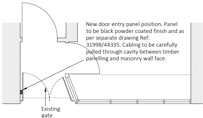
PARTIAL PLAN - AS PROPOSED 1:50@A3
