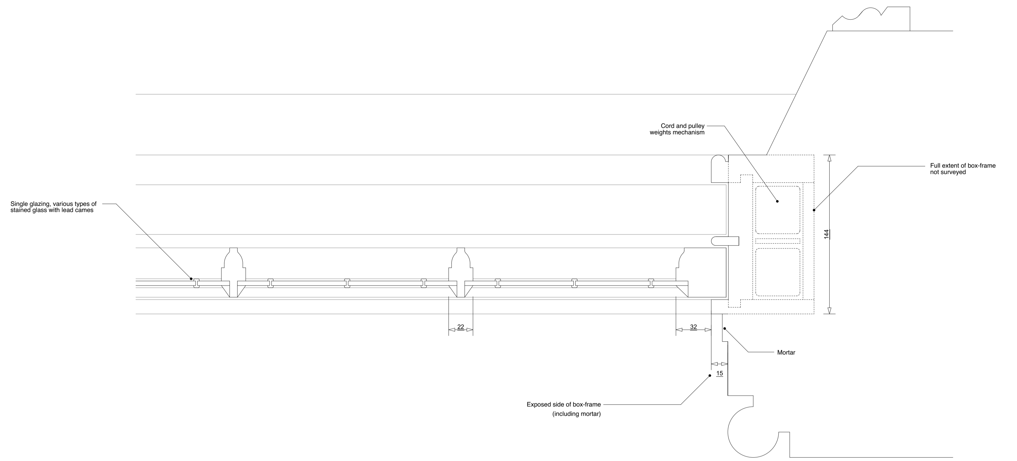
Existing Window Jamb Scale 1:2
