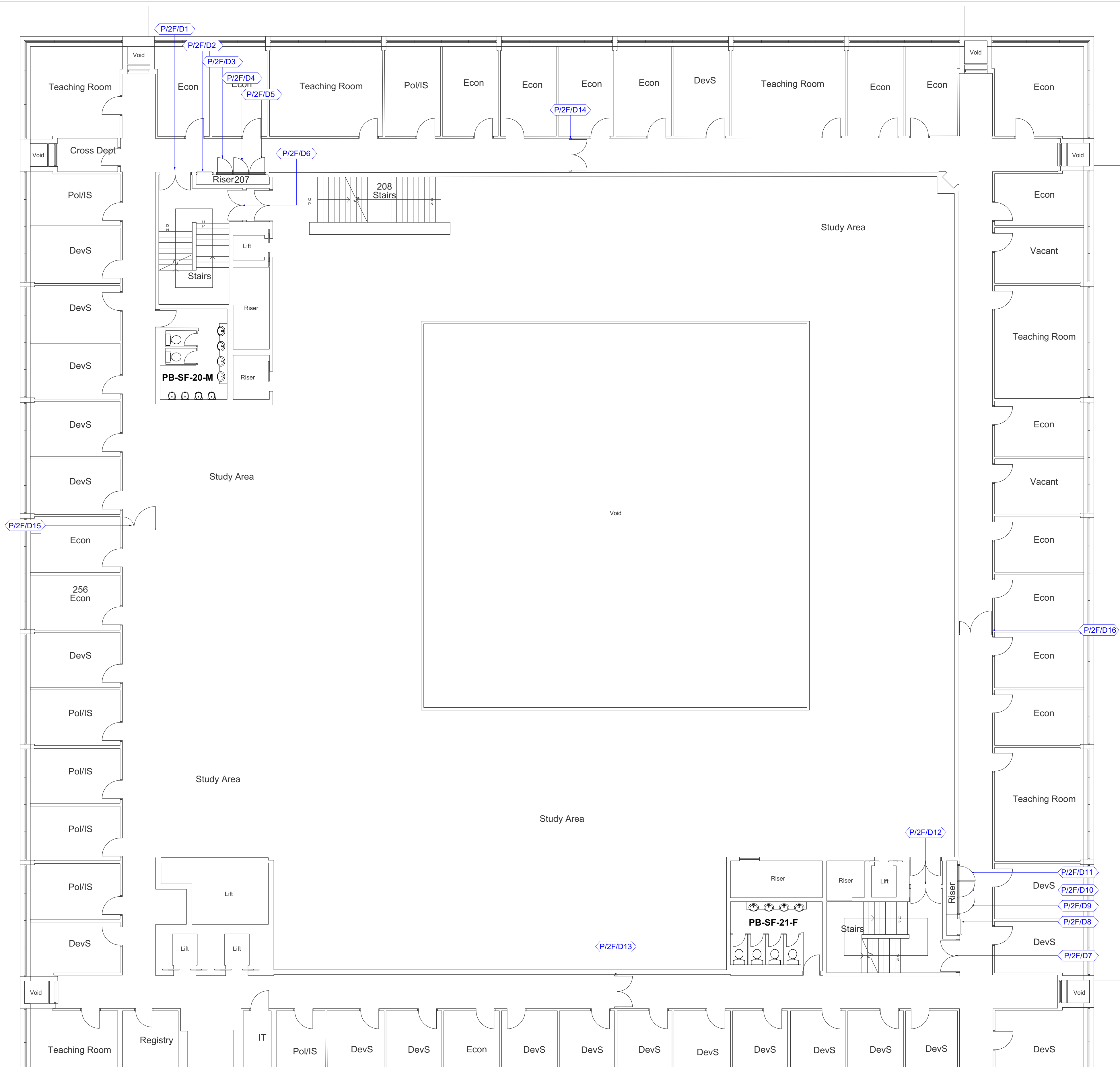
EXISTING SECOND FLOOR PLAN (1:100 @ A1)
