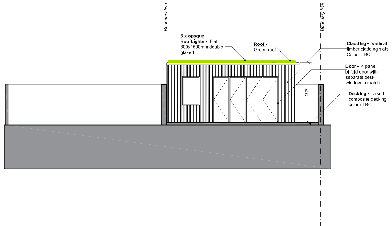
Proposed Front Elevation - Pavilion
