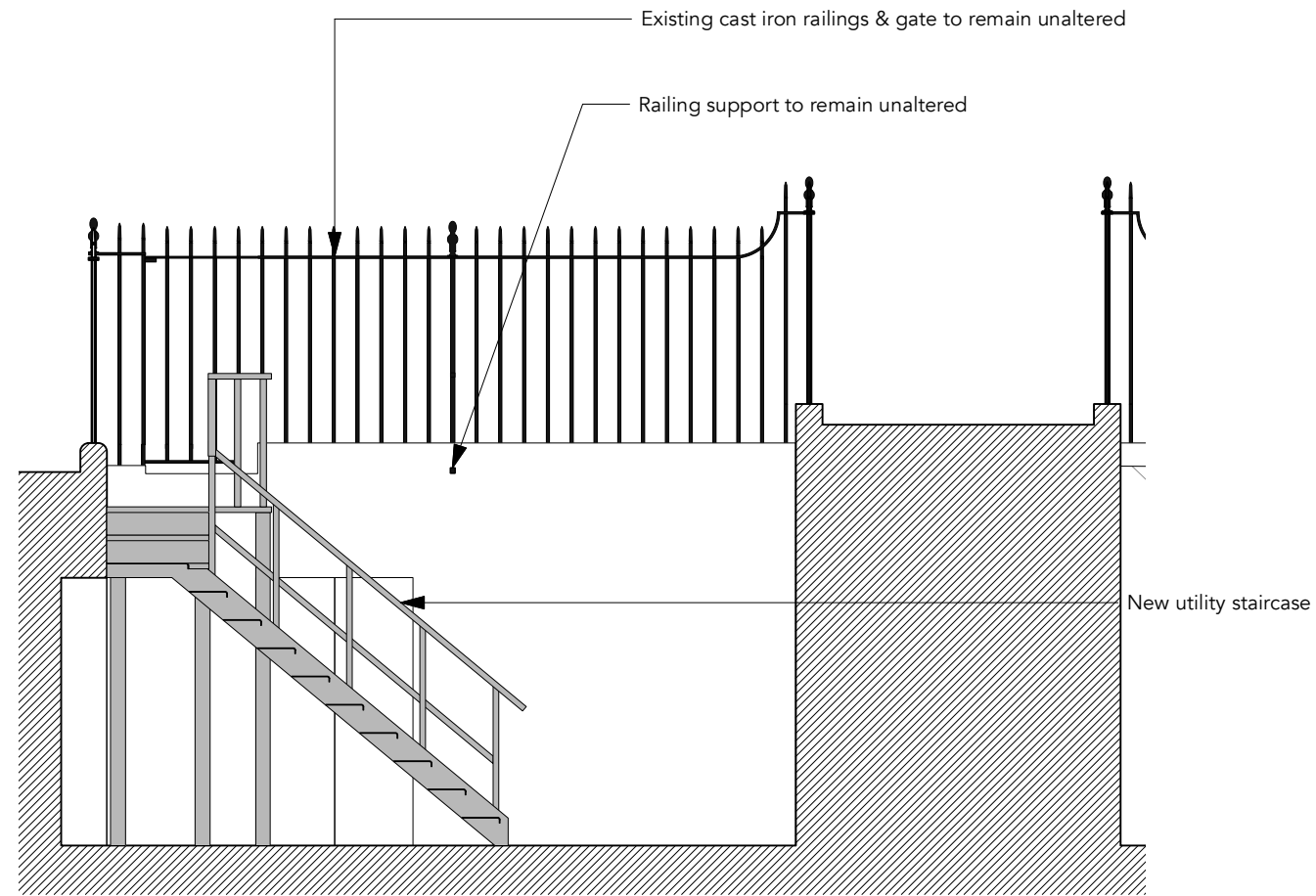
4 Proposed Section A-A 1:50
