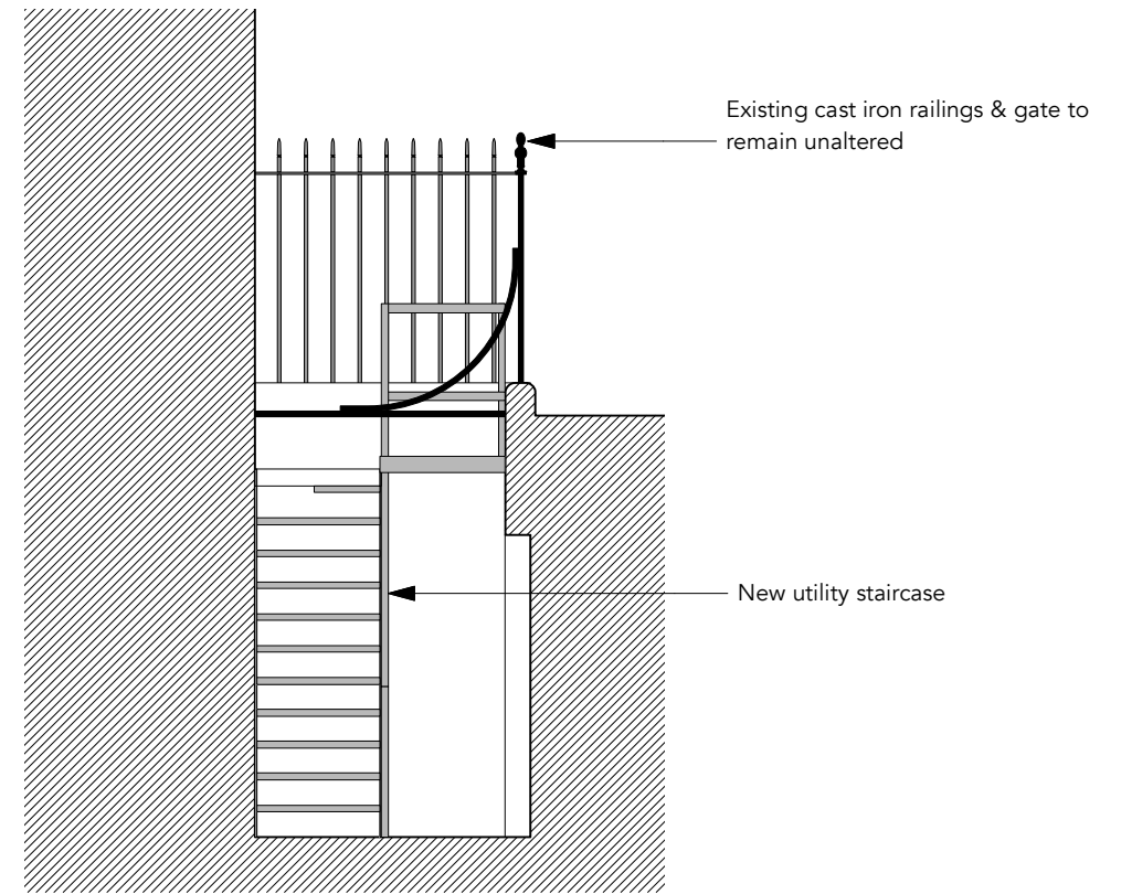
5 Proposed Section B-B 1:50
