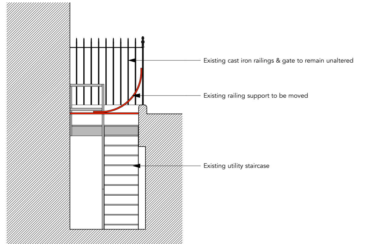
5 Existing Section B-B 1:50
