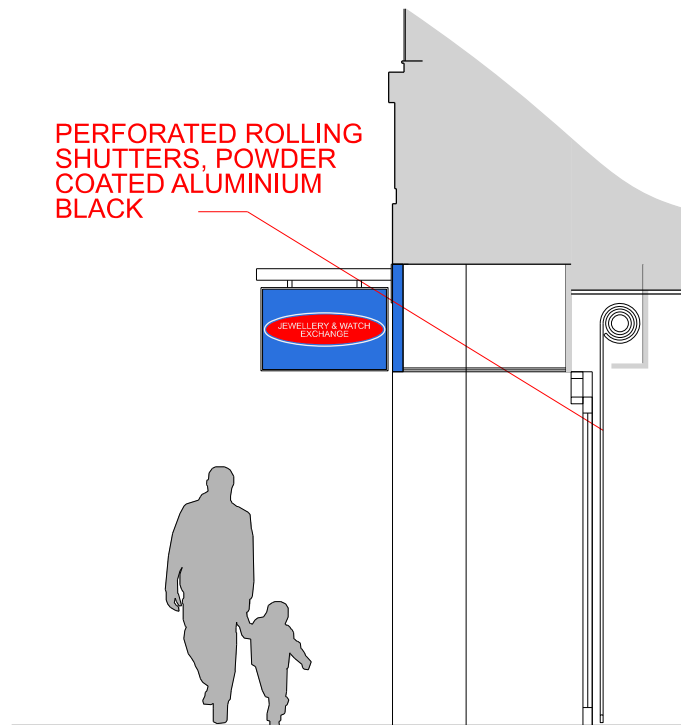
SECTION THROUGH ENTRANCE
