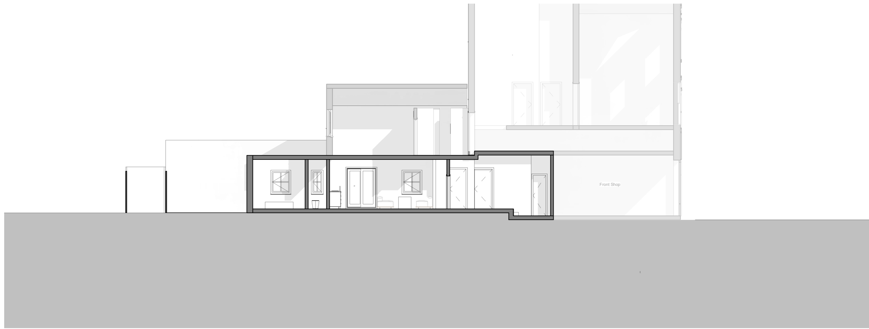
② Proposed Section A-A 1 : 100
