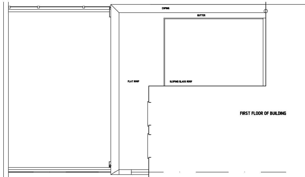
ROOF PLAN
