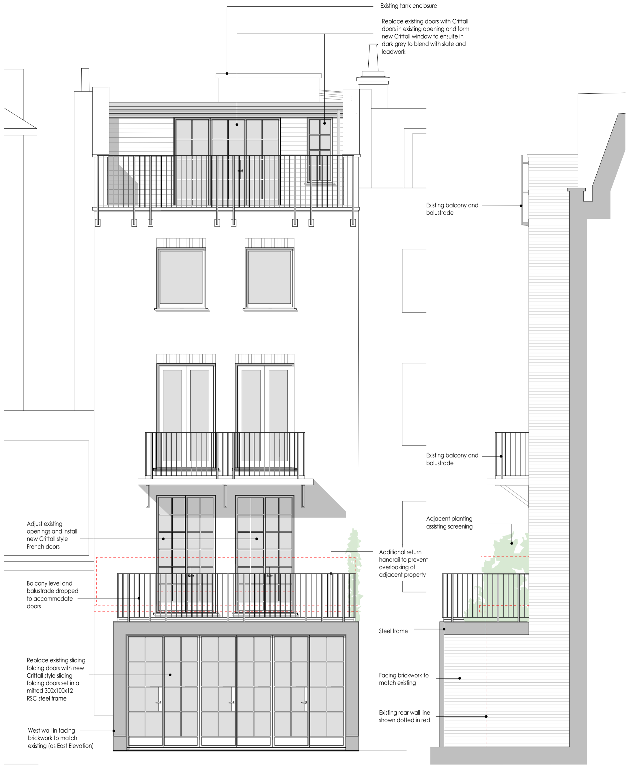
South Elevation (to Garden)
