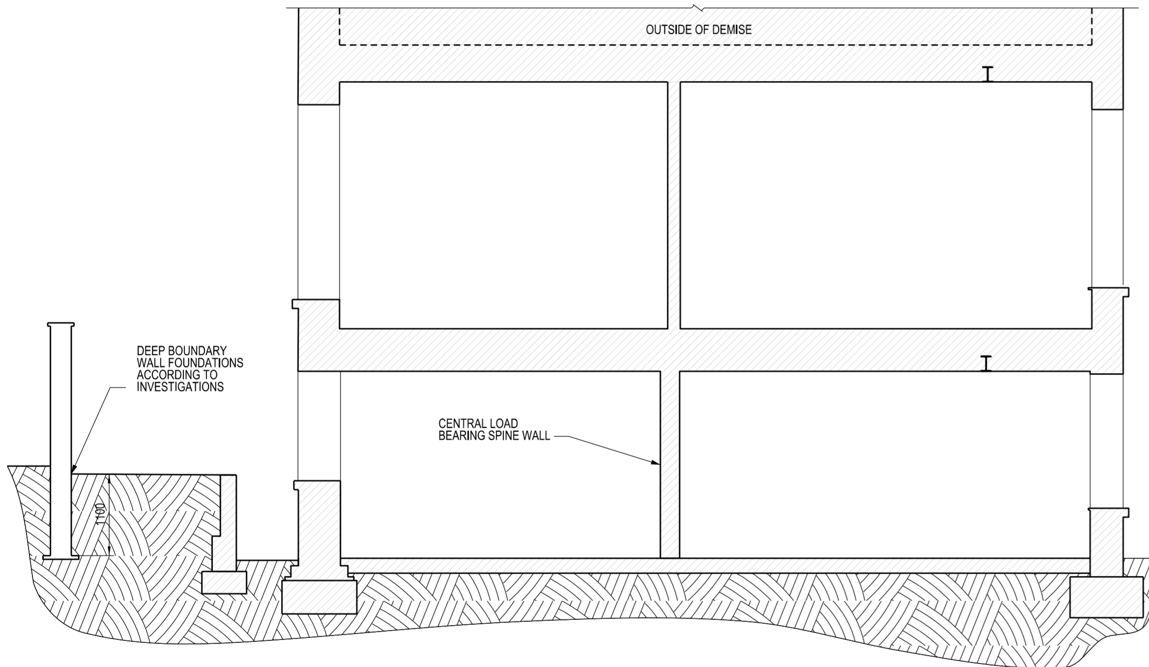
EXISTING SECTION 1-1
