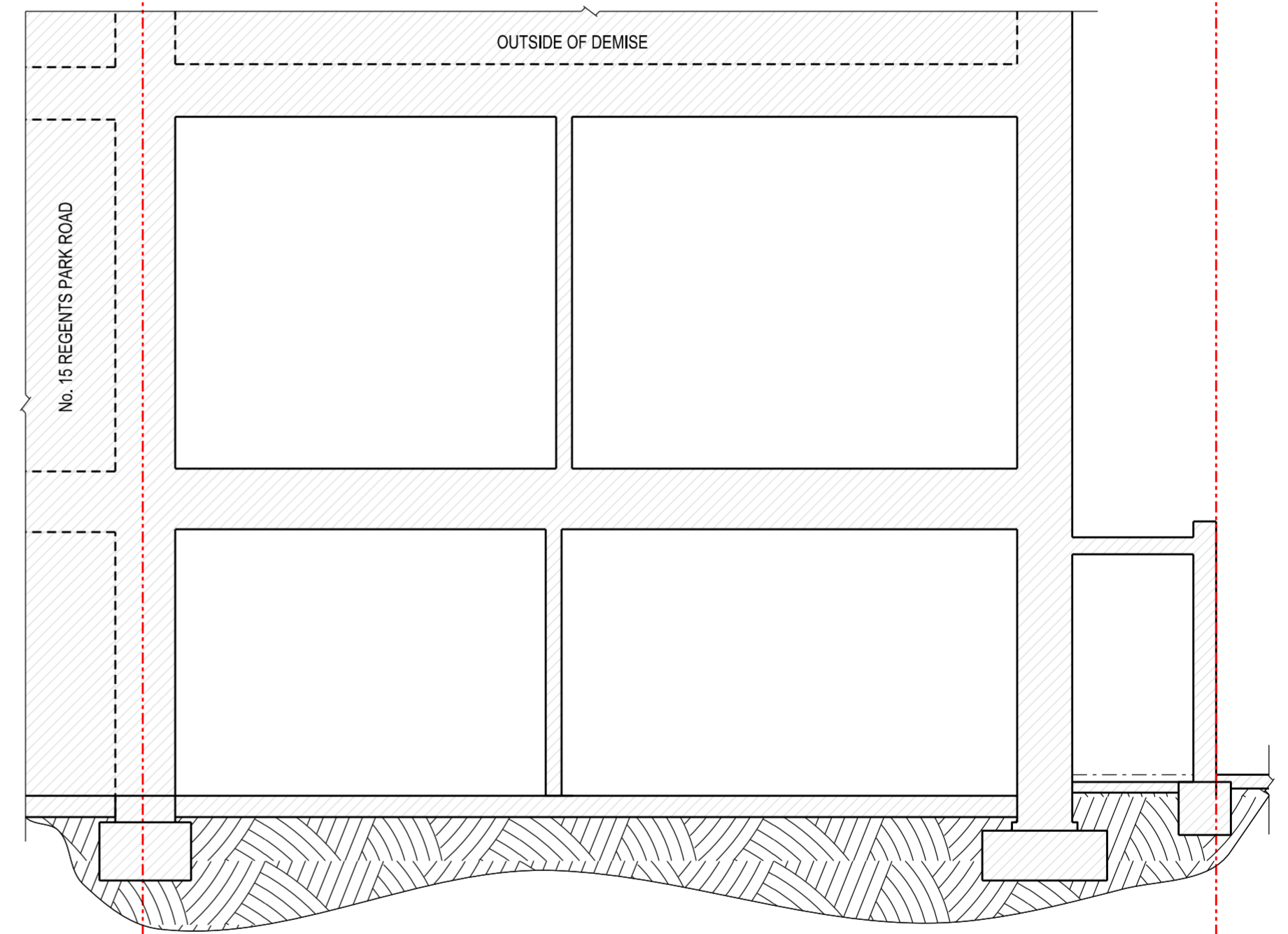
EXISTING SECTION 2-2
