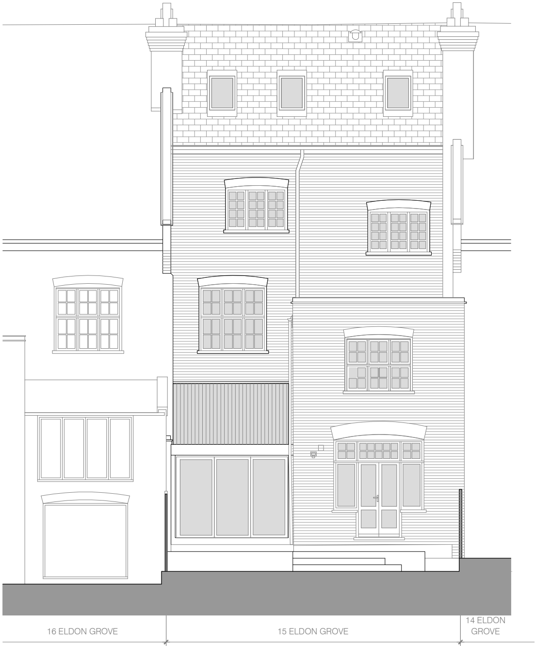
REAR ELEVATION
