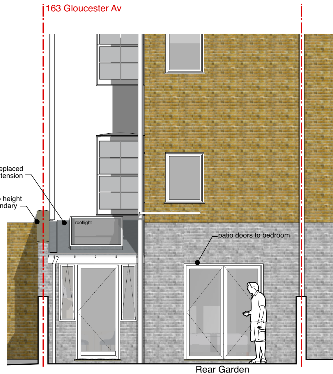
Section CC
