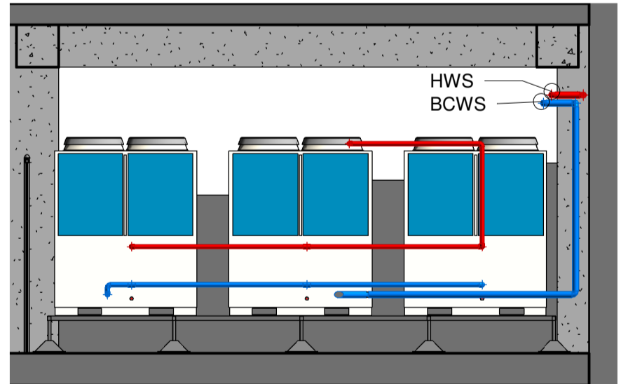
4 Section View- Heat Pumps 1 : 50
