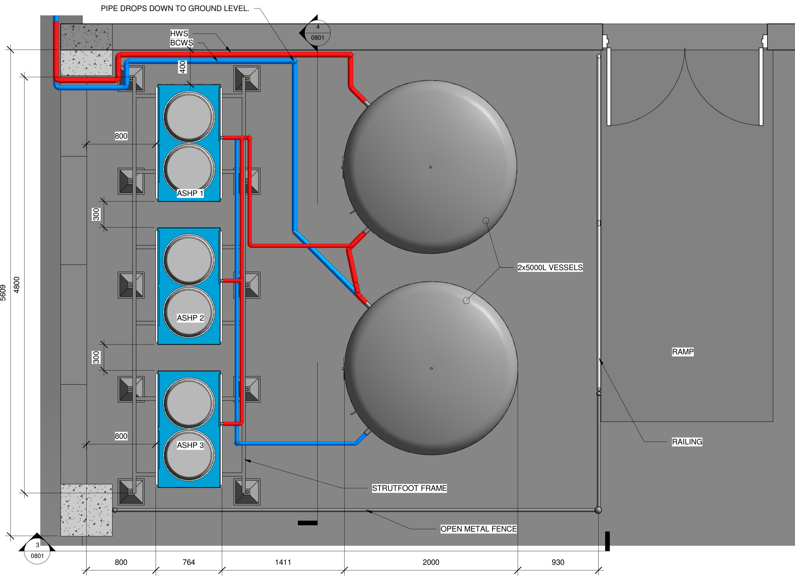
1 Plan View 1 : 25
