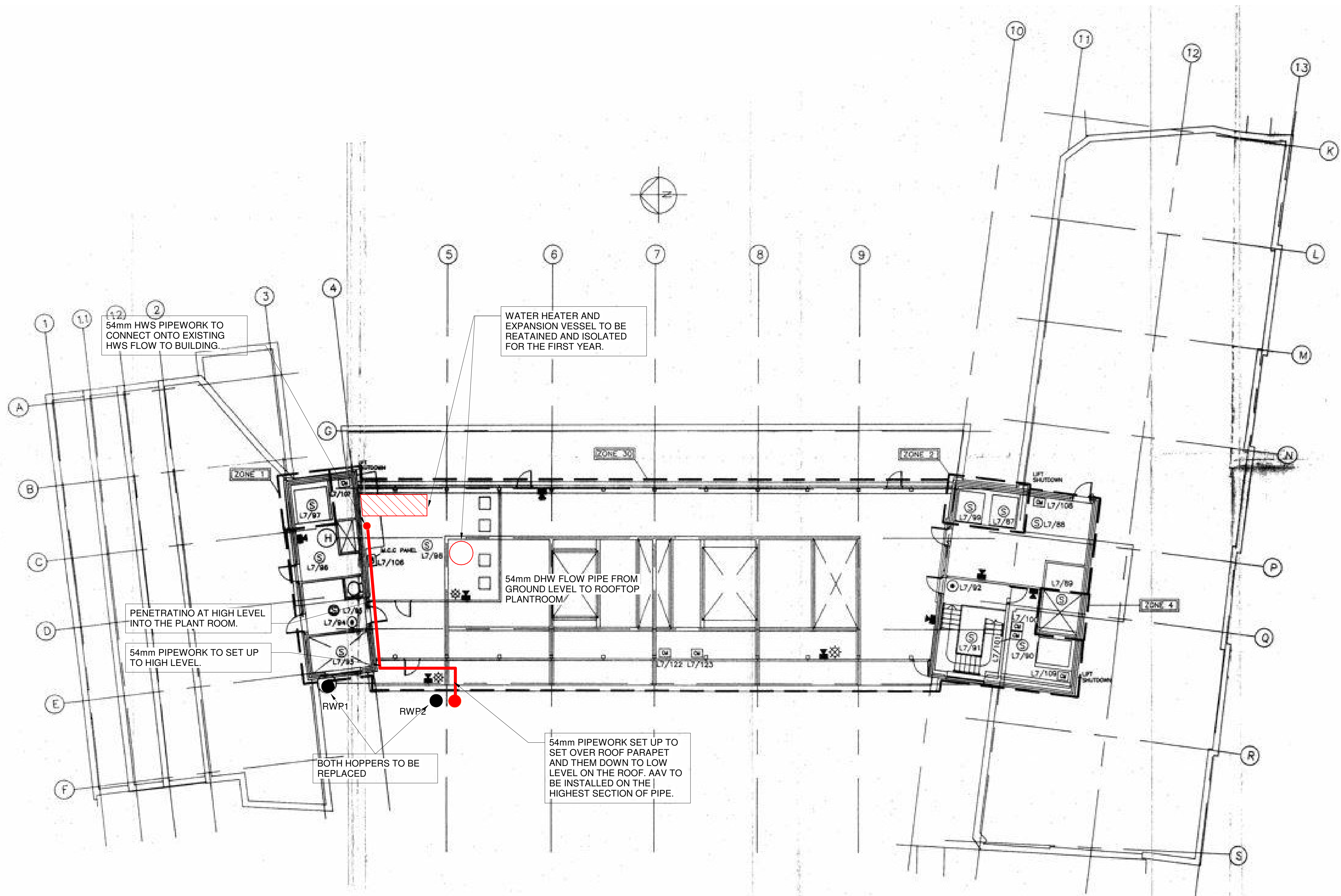
1 Roof Layout NTS
