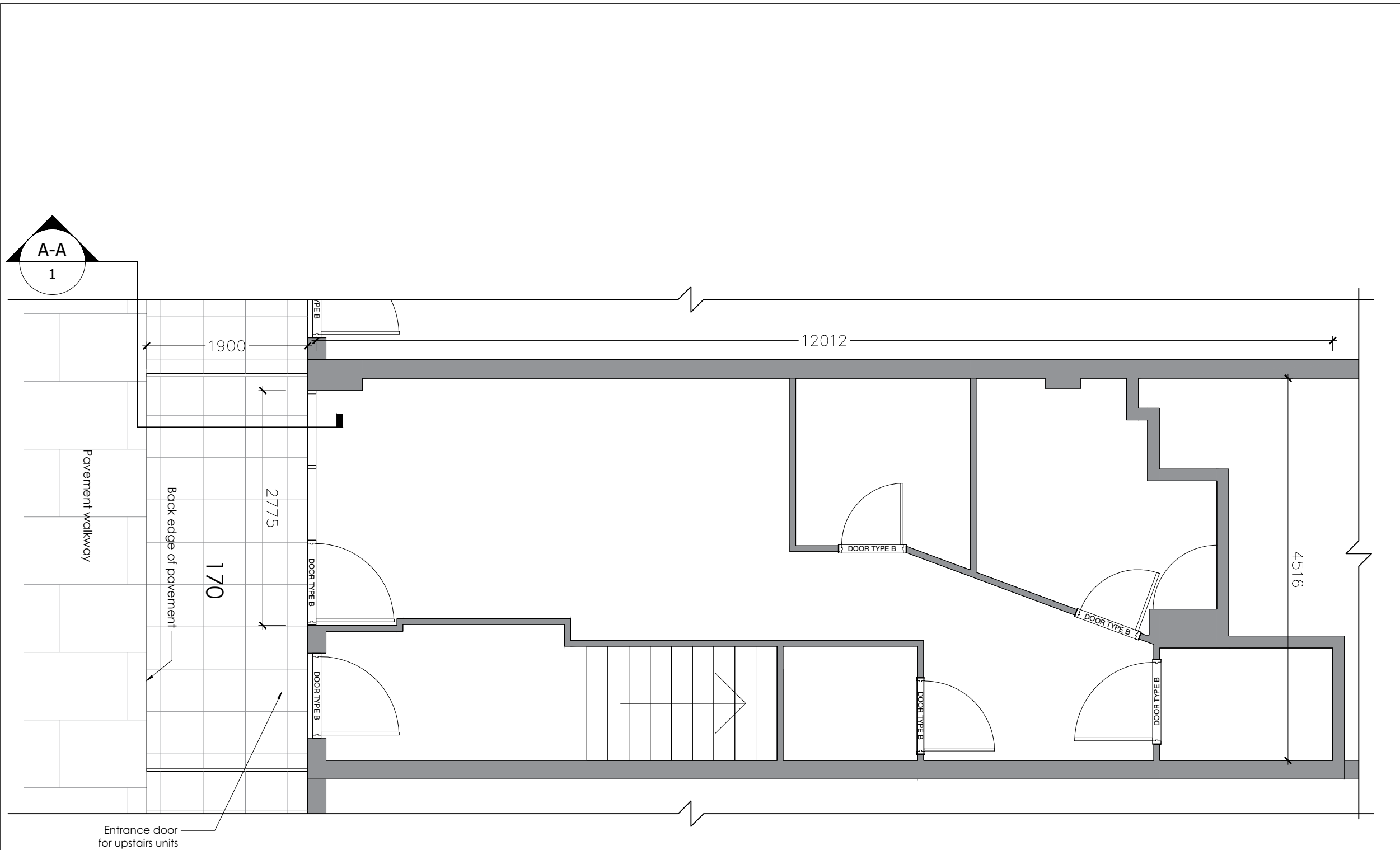
01 Existing Ground Floor Plan 1:50 @ A3
