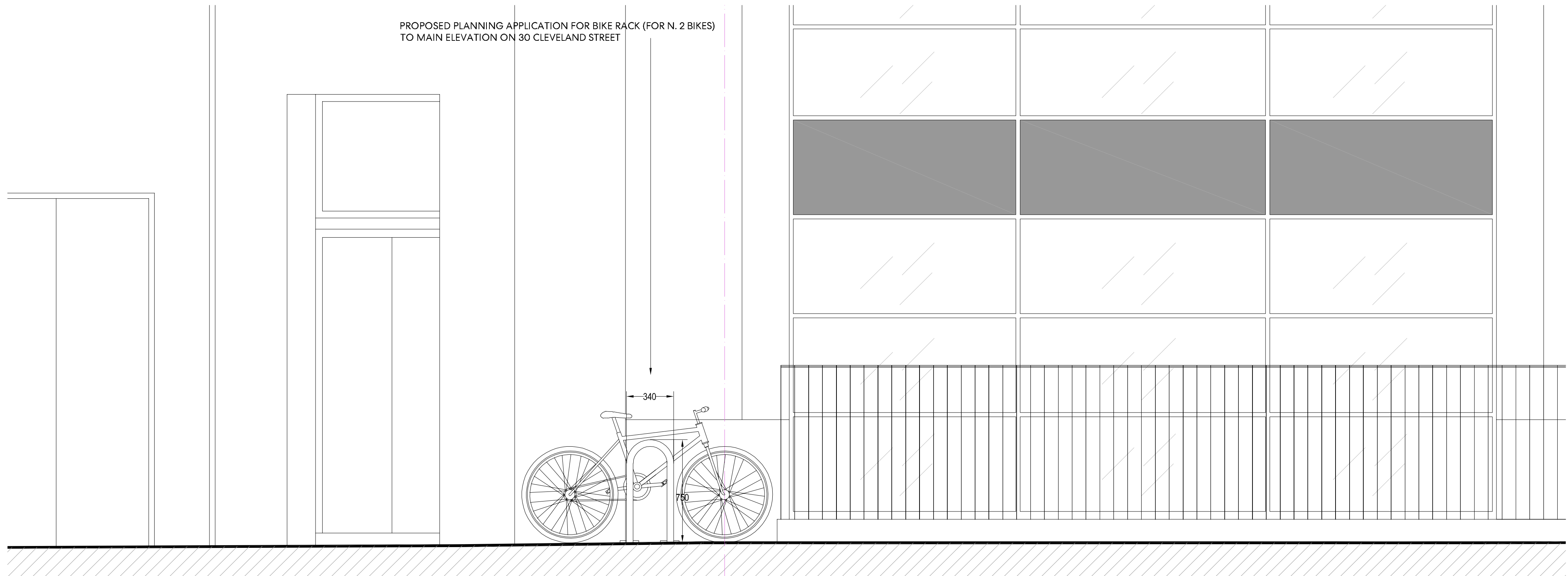
2 ENLARGED PROPOSED ELEVATION ON CLEVELAND STREET - LEVEL 00 1:20
