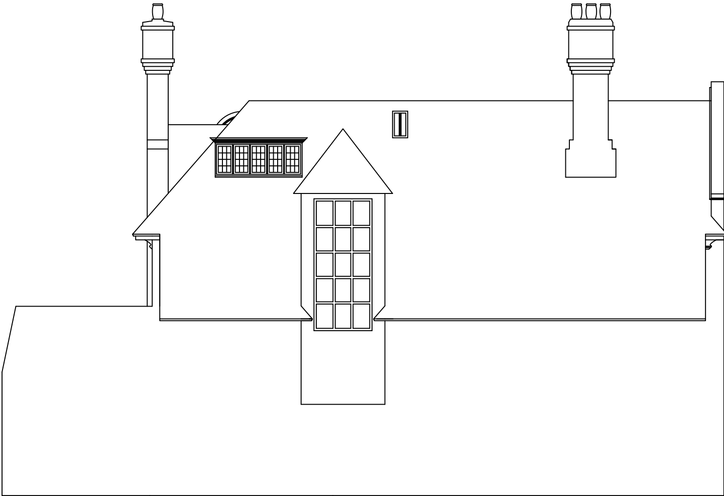
Rear Elevation Existing
