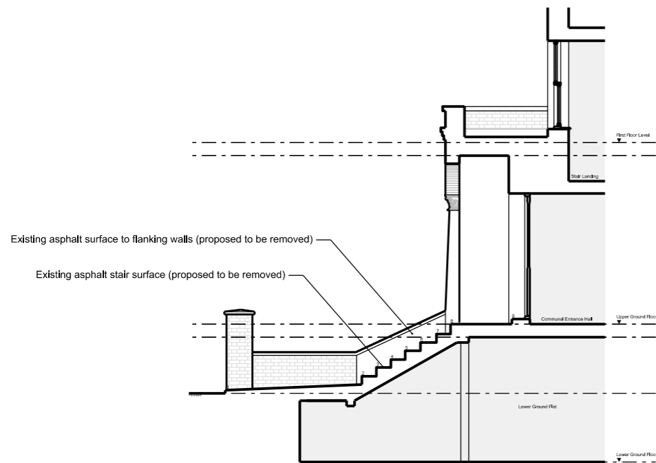
Existing Front Steps Section
