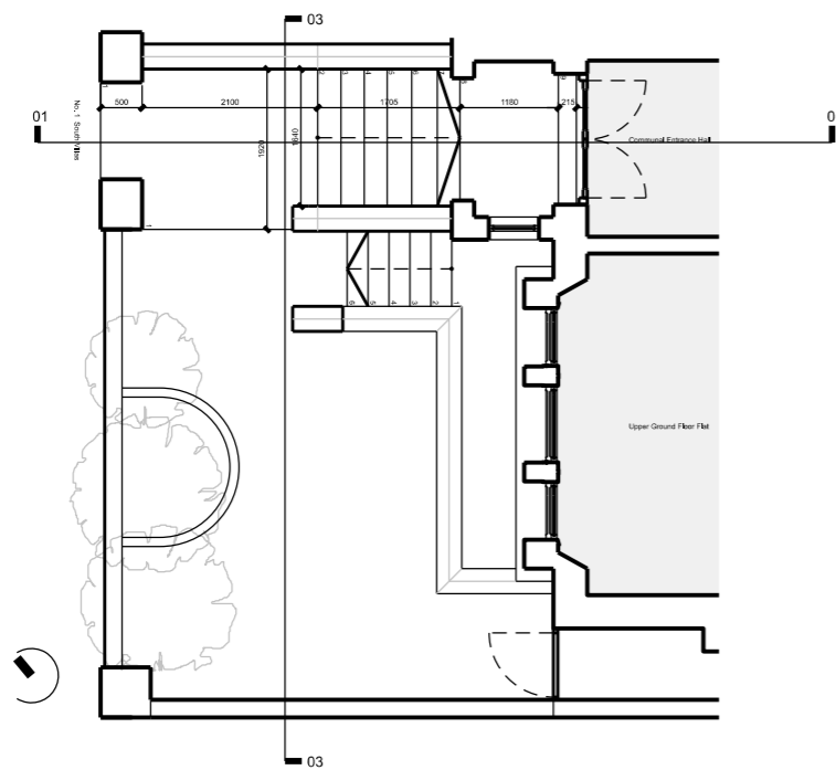
Existing Front Steps Plan
