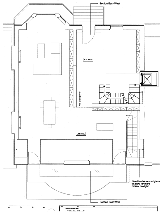
UPPER GROUND
