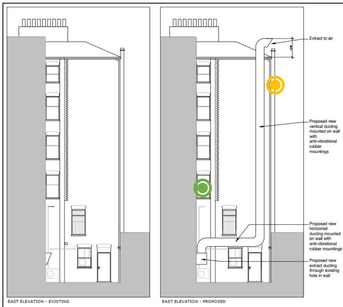
Figure 2.4 Proposed extract duct location, duct termination point and identified receiver 2 (Drawing Source: Tabitha Pope Architecture)
