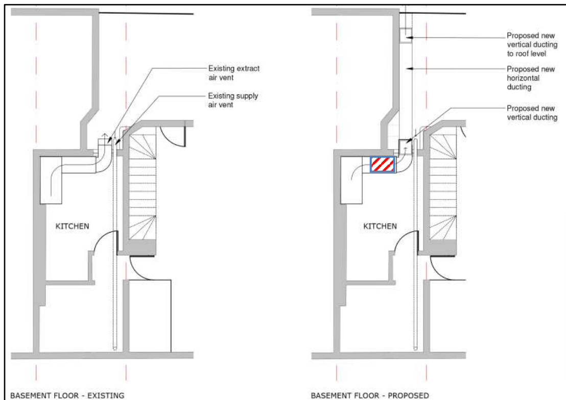
Figure 2.3 Proposed plant unit installation (Drawing Source: Tabitha Pope Architecture)
