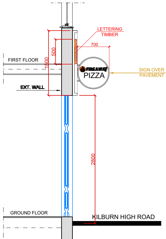
PROPOSED SECTION SCALE: 1/50
