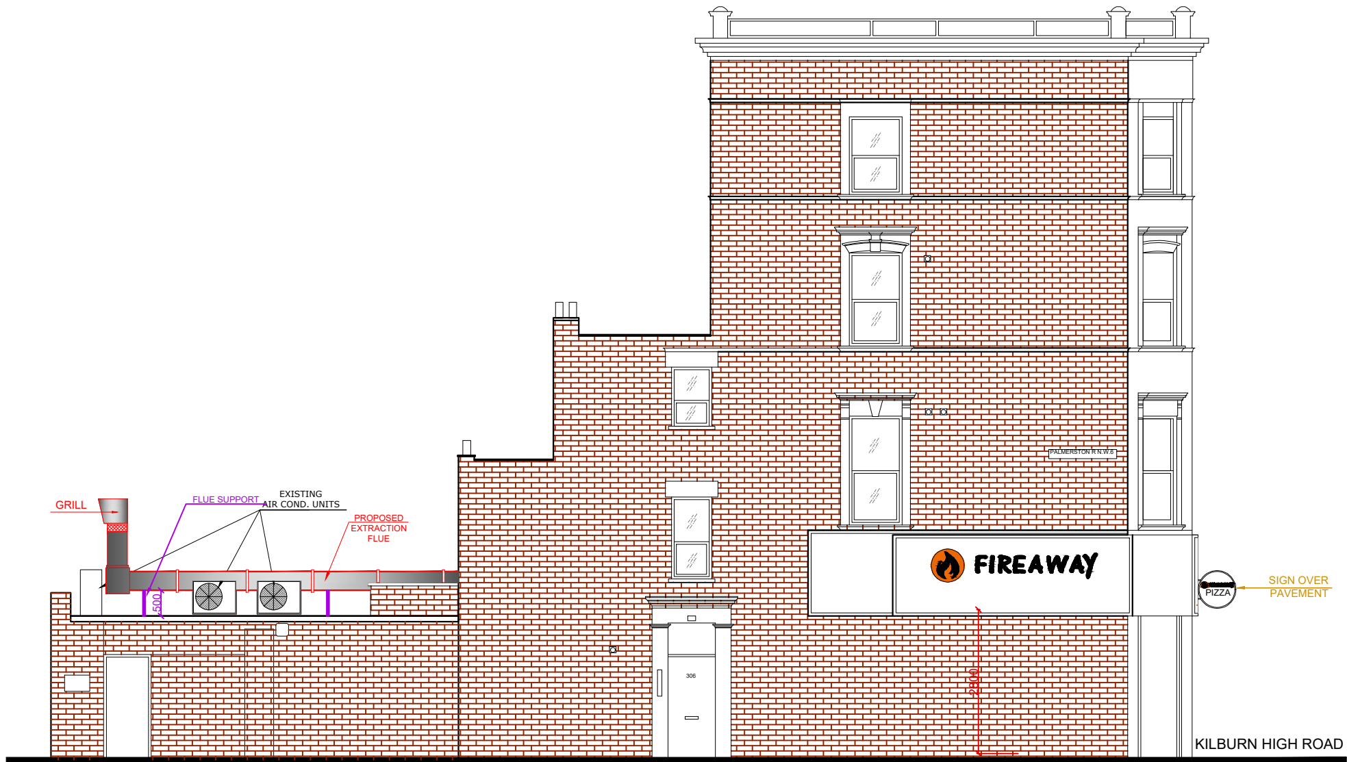
PROPOSED SIDE ELEVATION SCALE: 1/100 @A3
