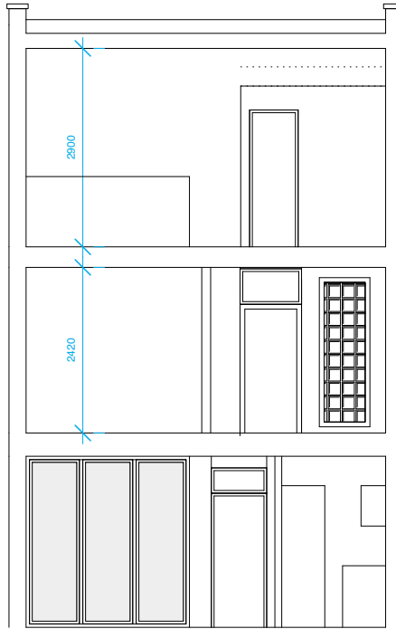
CROSS SECTION
