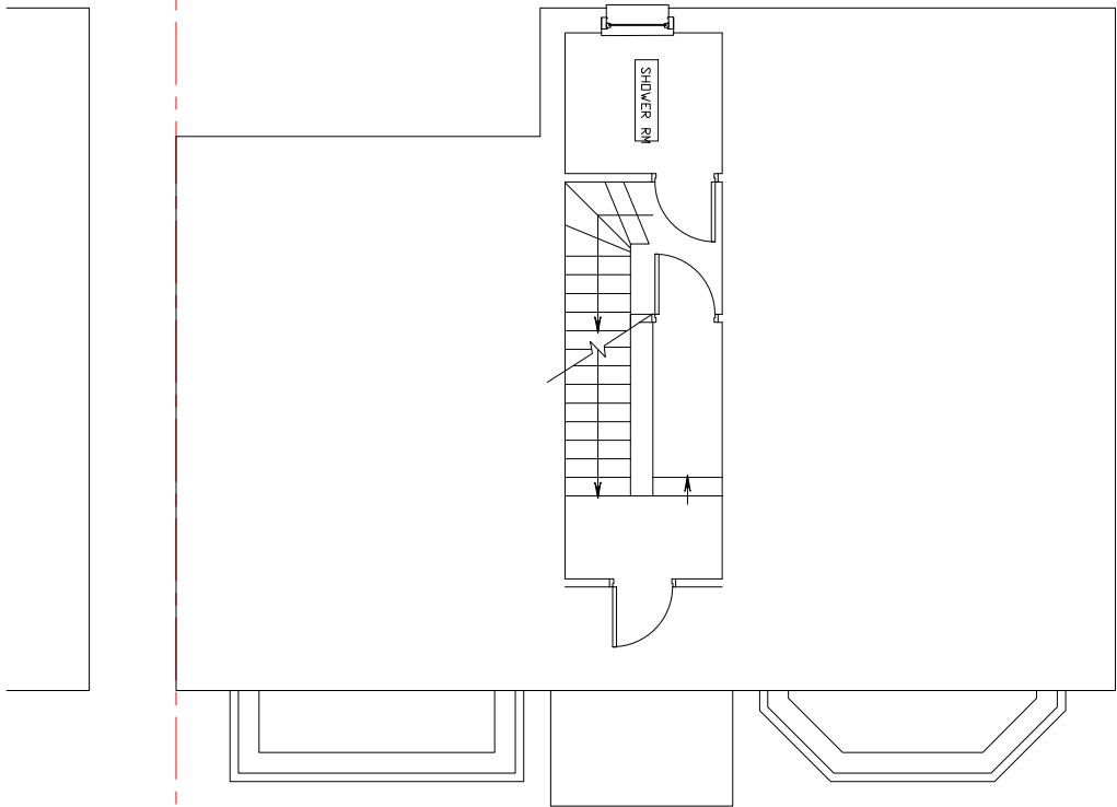
2 EXISTING 2ND FLOOR PLAN 1 : 100
