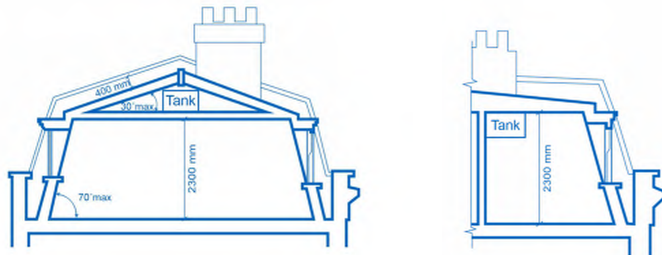
Mansard roof extensions: A. True mansard (left); B. Flat topped mansard
