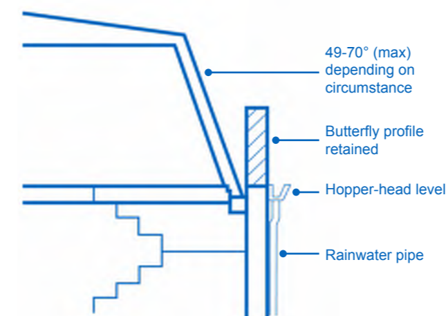
Example of mansard on butterfly roof
