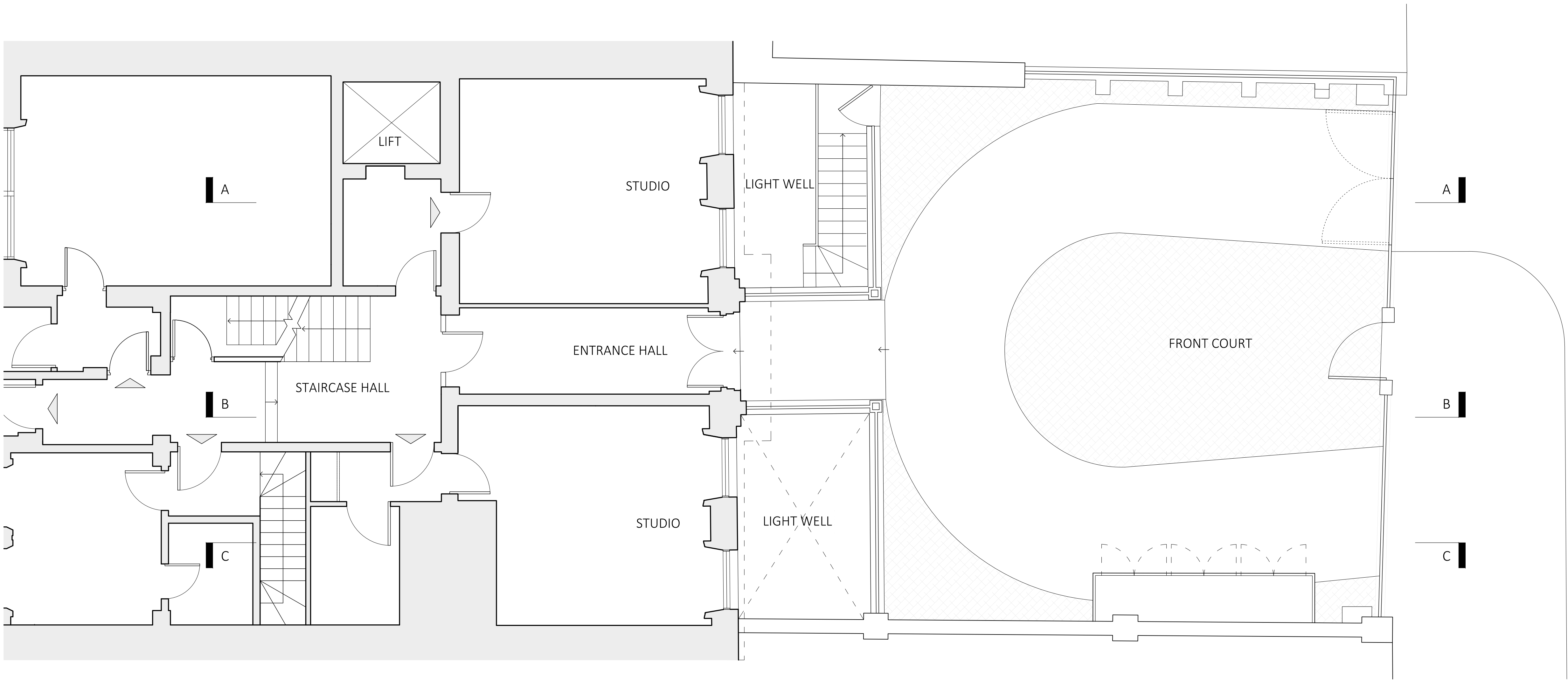
GROUND FLOOR AS EXISTING
