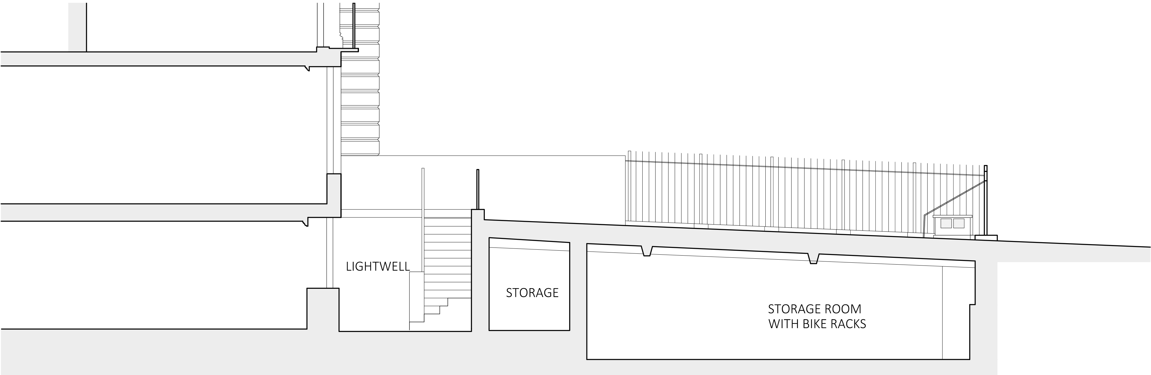
SECTION AA AS EXISTING
