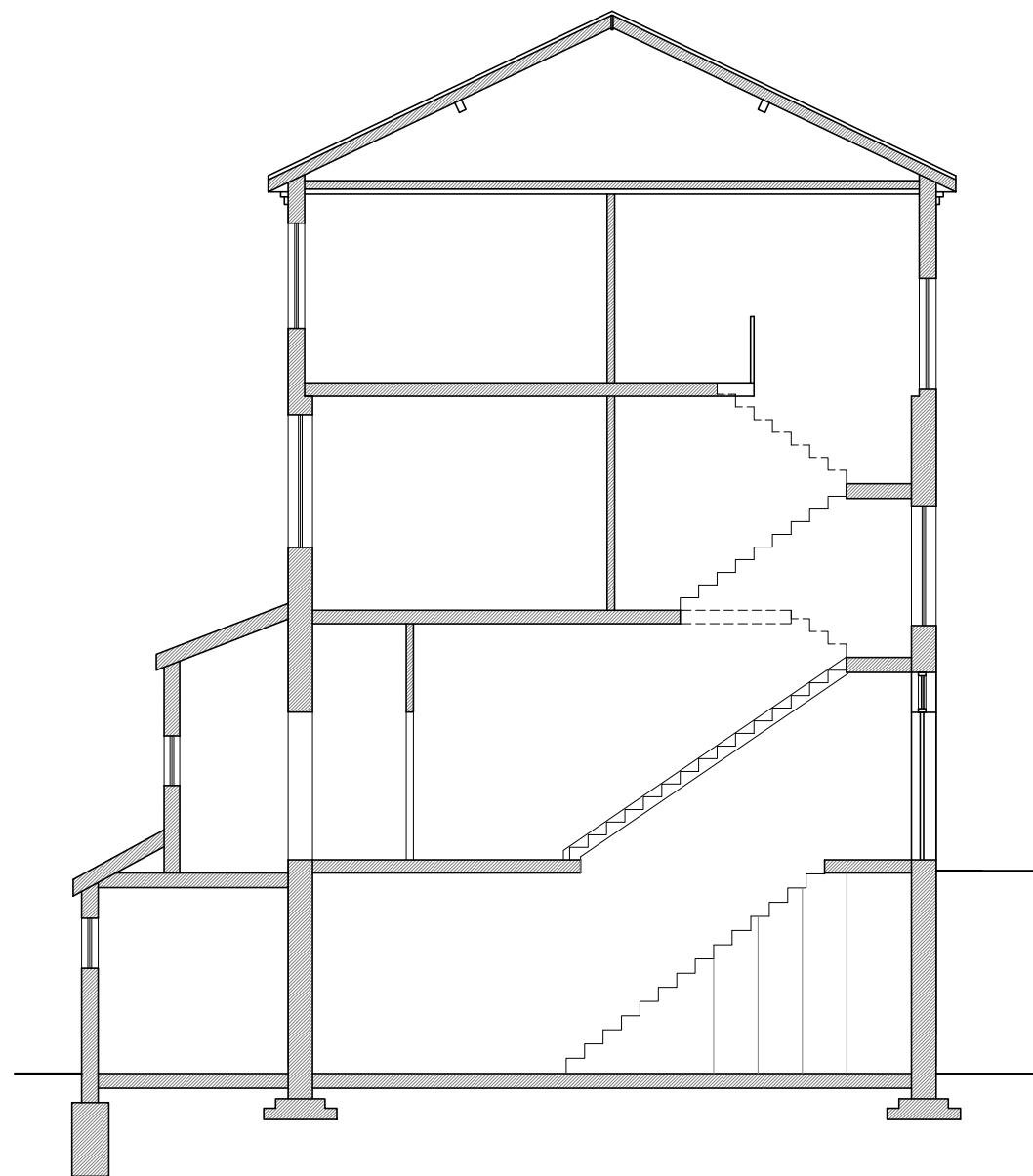
SECTION B-B
