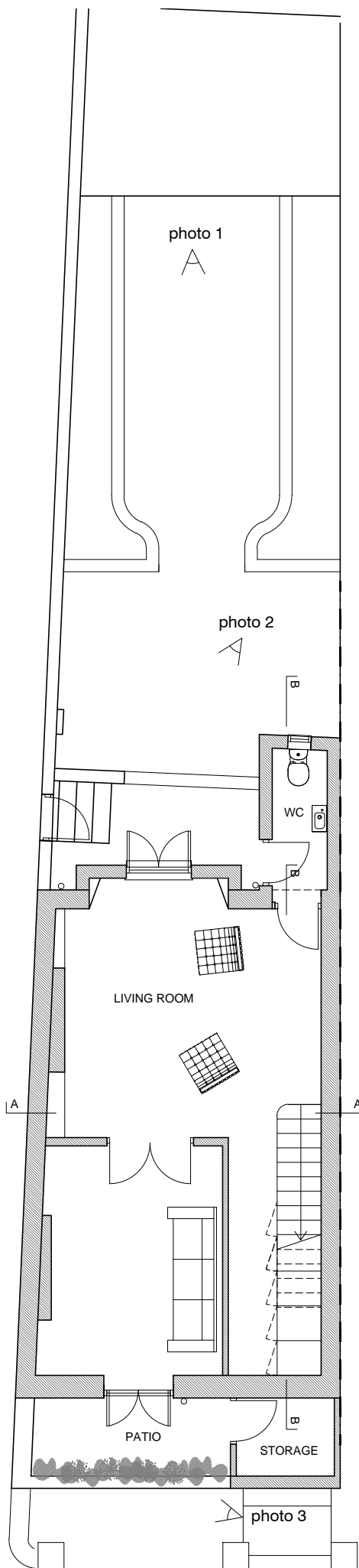
LOWER GROUND FLOOR PLAN
