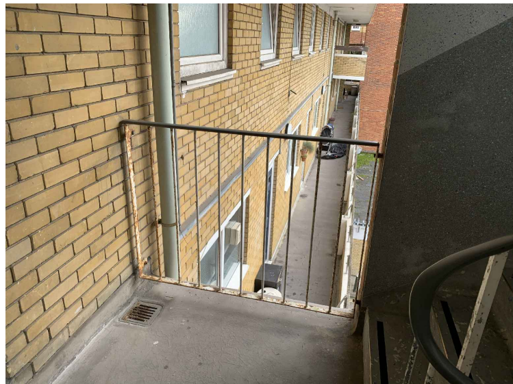
PHOTO 'D' SHOWING THIRD FLOOR SAFETY HANDRAIL.
