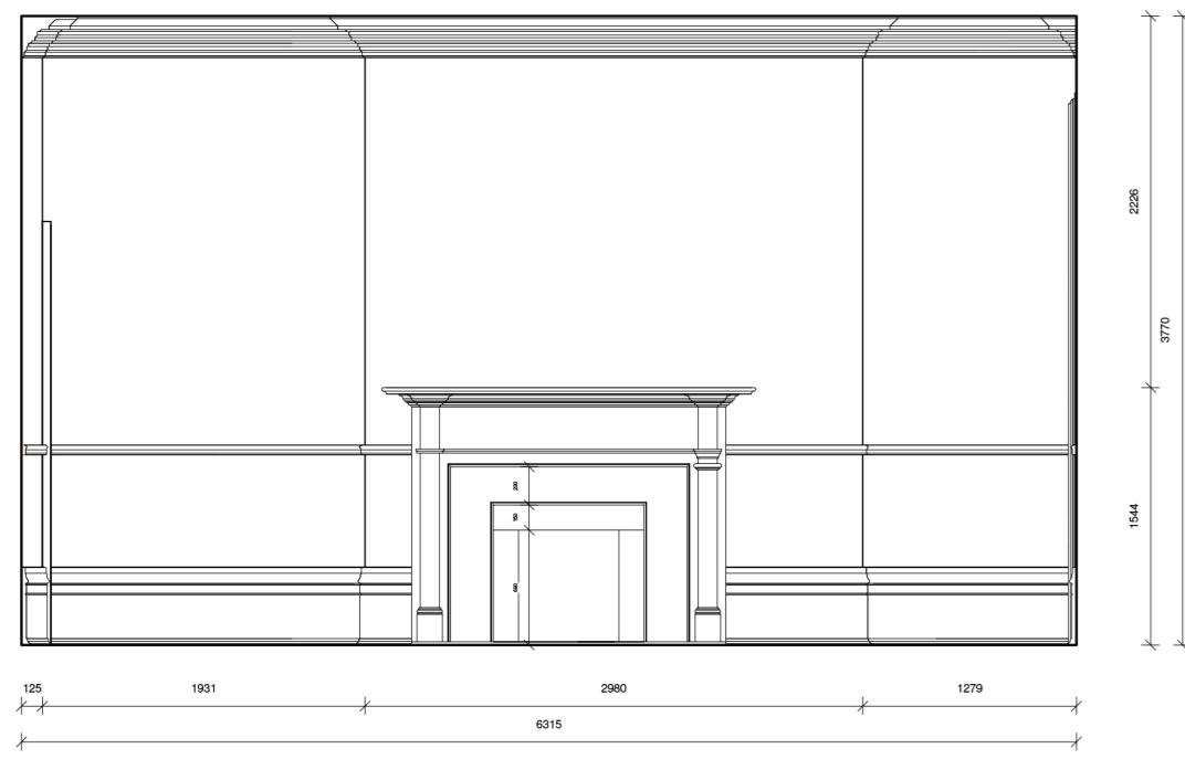
2 Elevation 2 - Existing 1 : 50
