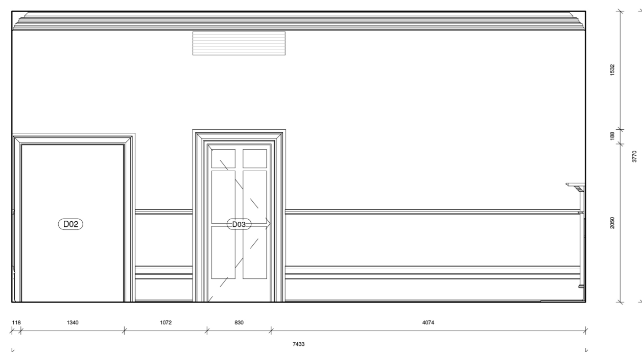
4 Elevation 4 - Existing 1 : 50
