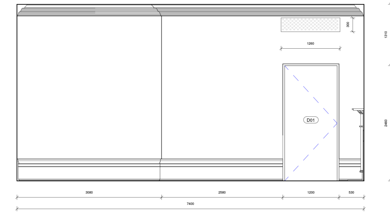
1 Elevation 1 - Proposed 1 : 50
