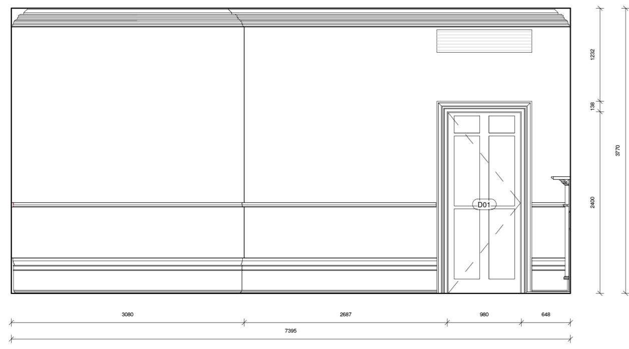
1 Elevation 1 - Existing 1 : 50
