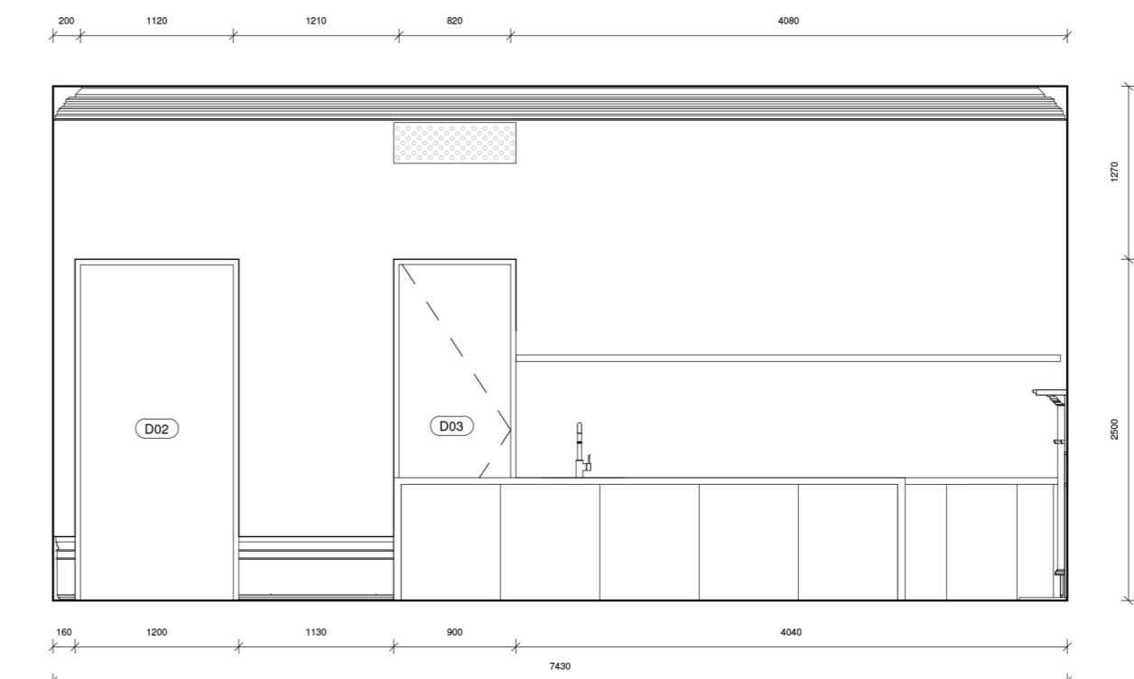
4 Elevation 4 - Proposed 1 : 50
