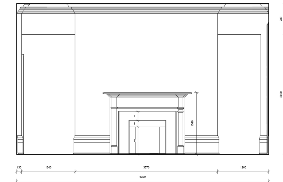
2 Elevation 2 - Proposed 1 : 50
