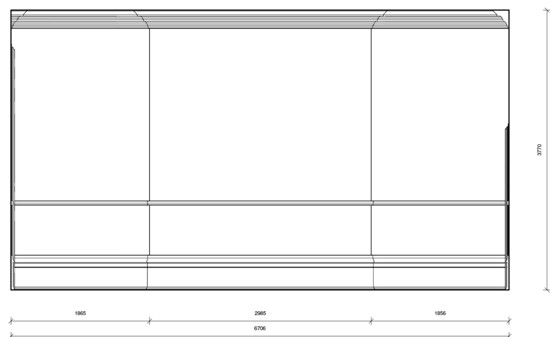
3 Elevation 3 - Existing 1 : 50
