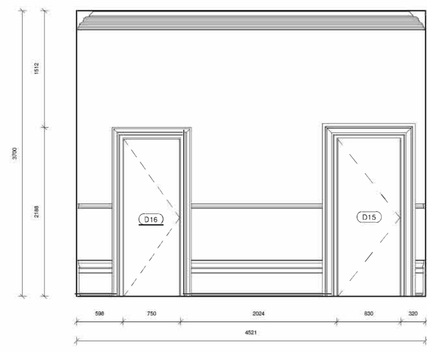
38 Elevation 19 - Existing 1 : 50
