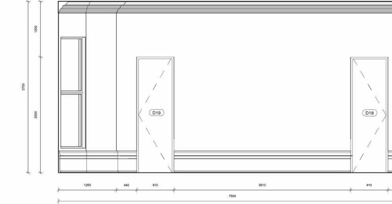
20 Elevation 21 - Proposed 1 : 50
