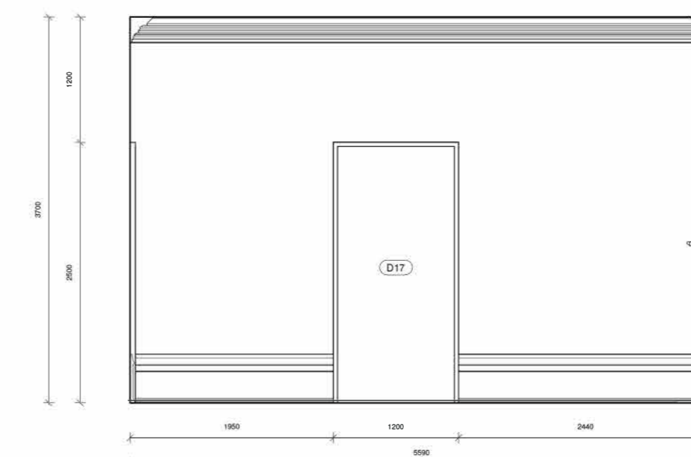
21 Elevation 20 - Proposed 1 : 50
