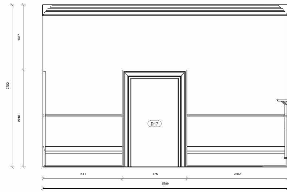
39 Elevation 20 - Existing 1 : 50
