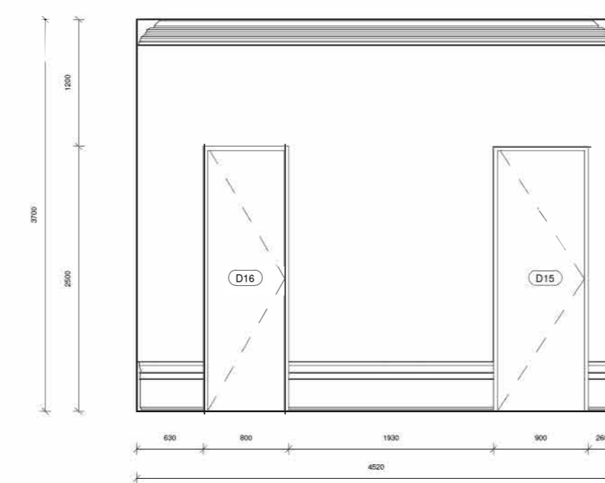
19 Elevation 19 - Proposed 1 : 50
