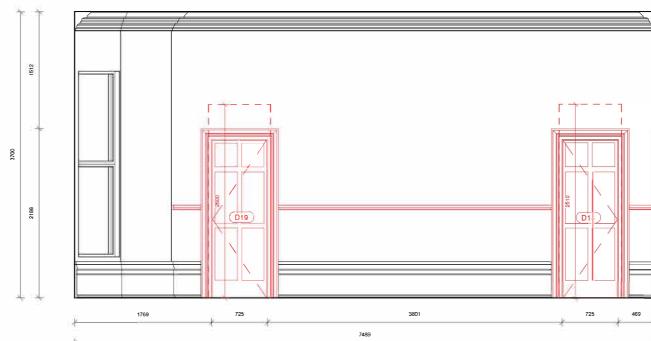
43 Elevation 21 - Demo 1 : 50
