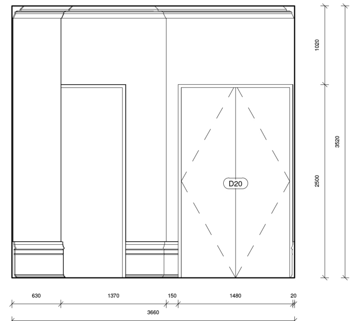
14 Elevation 14 - Proposed 1 : 50
