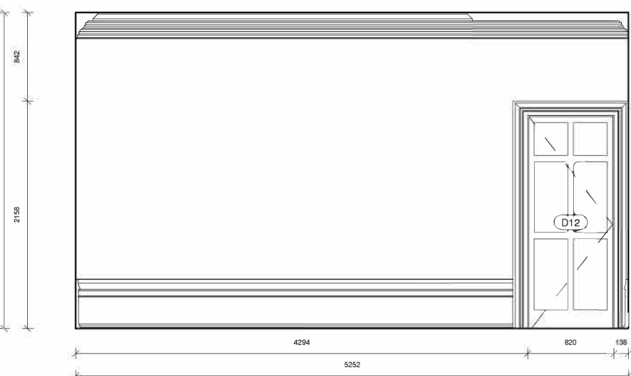
32 Elevation 18 - Existing 1 : 50
