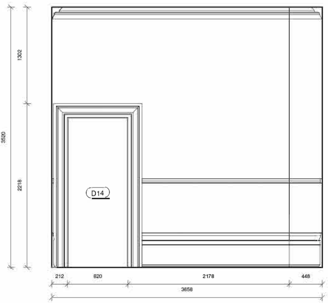
29 Elevation 15 - Existing 1 : 50
