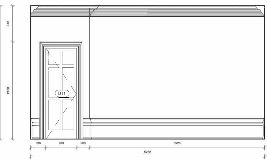
31 Elevation 17 - Existing 1 : 50
