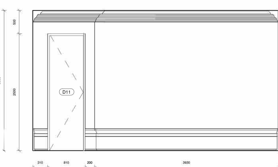
18 Elevation 17 - Proposed 1 : 50
