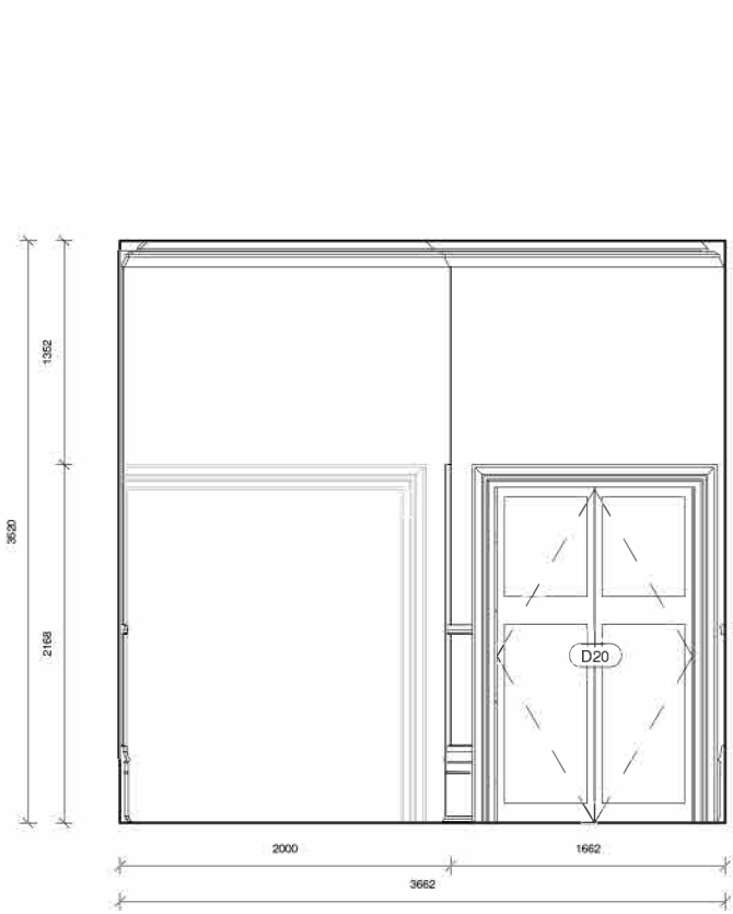
28 Elevation 14 - Existing 1 : 50
