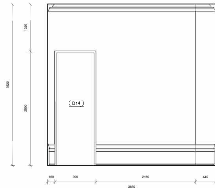
15 Elevation 15 - Proposed 1 : 50
