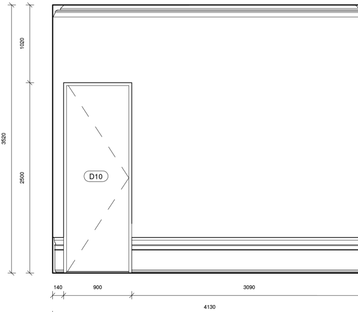
12 Elevation 12 - Proposed 1 : 50
