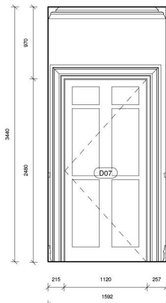
17 Elevation 9 - Existing 1 : 50
