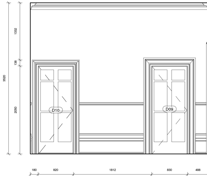
20 Elevation 12 - Existing 1 : 50
