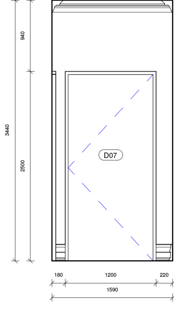
9 Elevation 9 - Proposed 1 : 50
