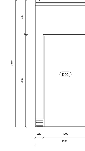
10 Elevation 10 - Proposed 1 : 50
