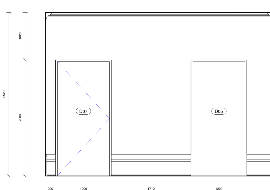
13 Elevation 13 - Proposed 1 : 50
