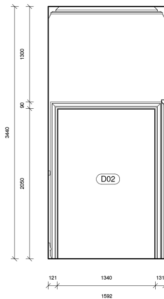
18 Elevation 10 - Existing 1 : 50
