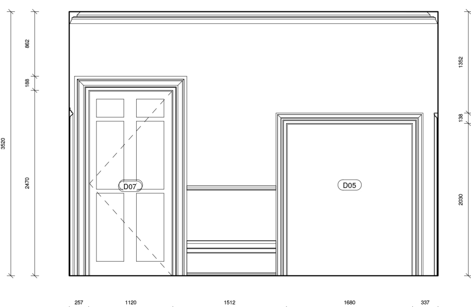
21 Elevation 13 - Existing 1 : 50
