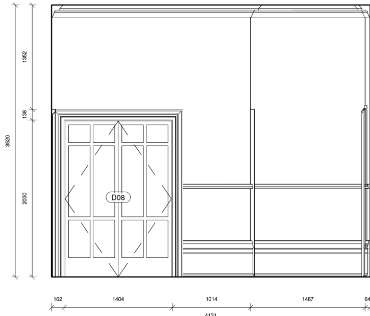
19 Elevation 11 - Existing 1 : 50
