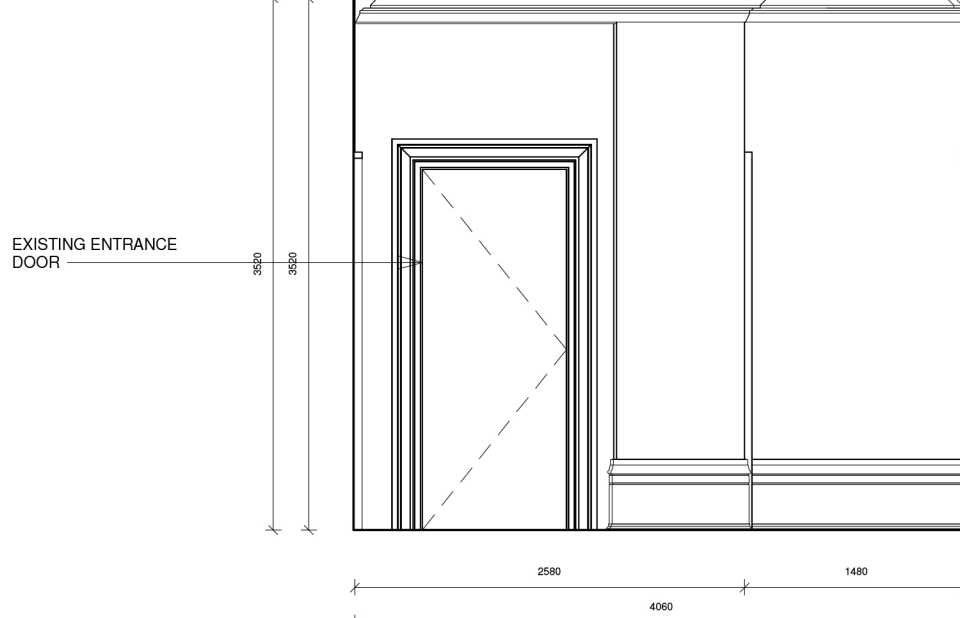
11 Elevation 11 - Proposed 1 : 50
