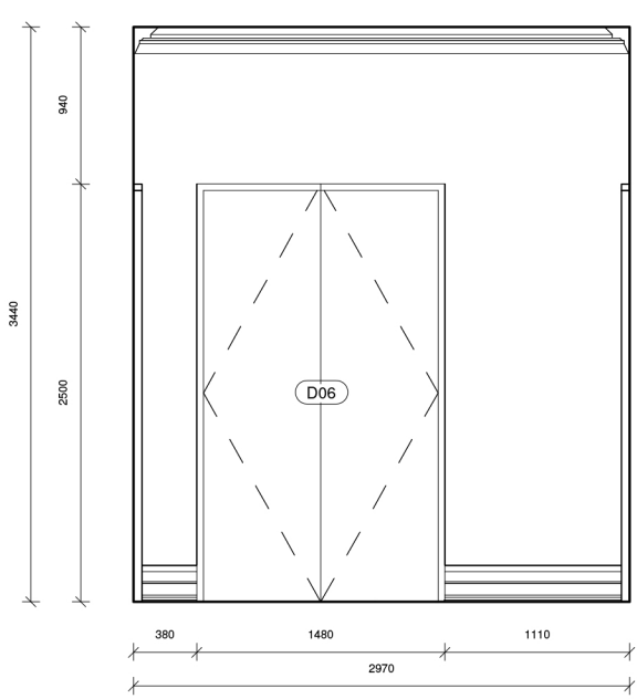
8 Elevation 8 - Proposed 1 : 50
