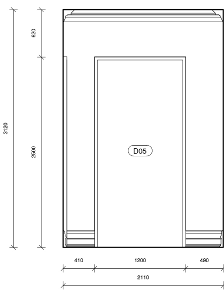
6 Elevation 6 - Proposed 1 : 50
