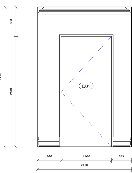
7 Elevation 7 - Proposed 1 : 50
