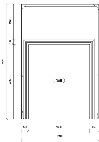
10 Elevation 6 - Existing 1 : 50
