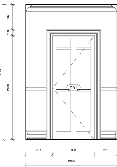
11 Elevation 7 - Existing 1 : 50
