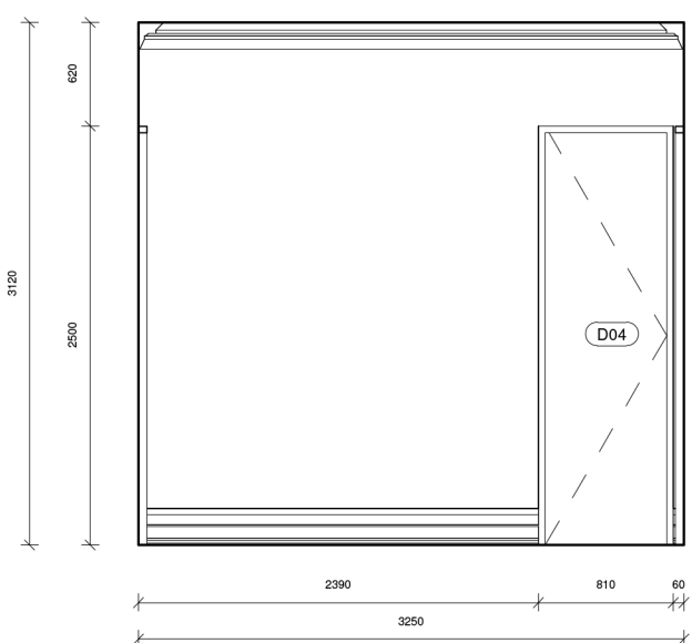
5 Elevation 5 - Proposed 1 : 50
