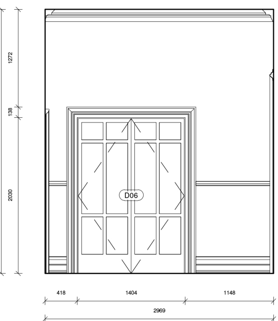
12 Elevation 8 - Existing 1 : 50
