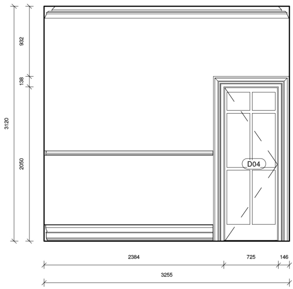
9 Elevation 5 - Existing 1 : 50
