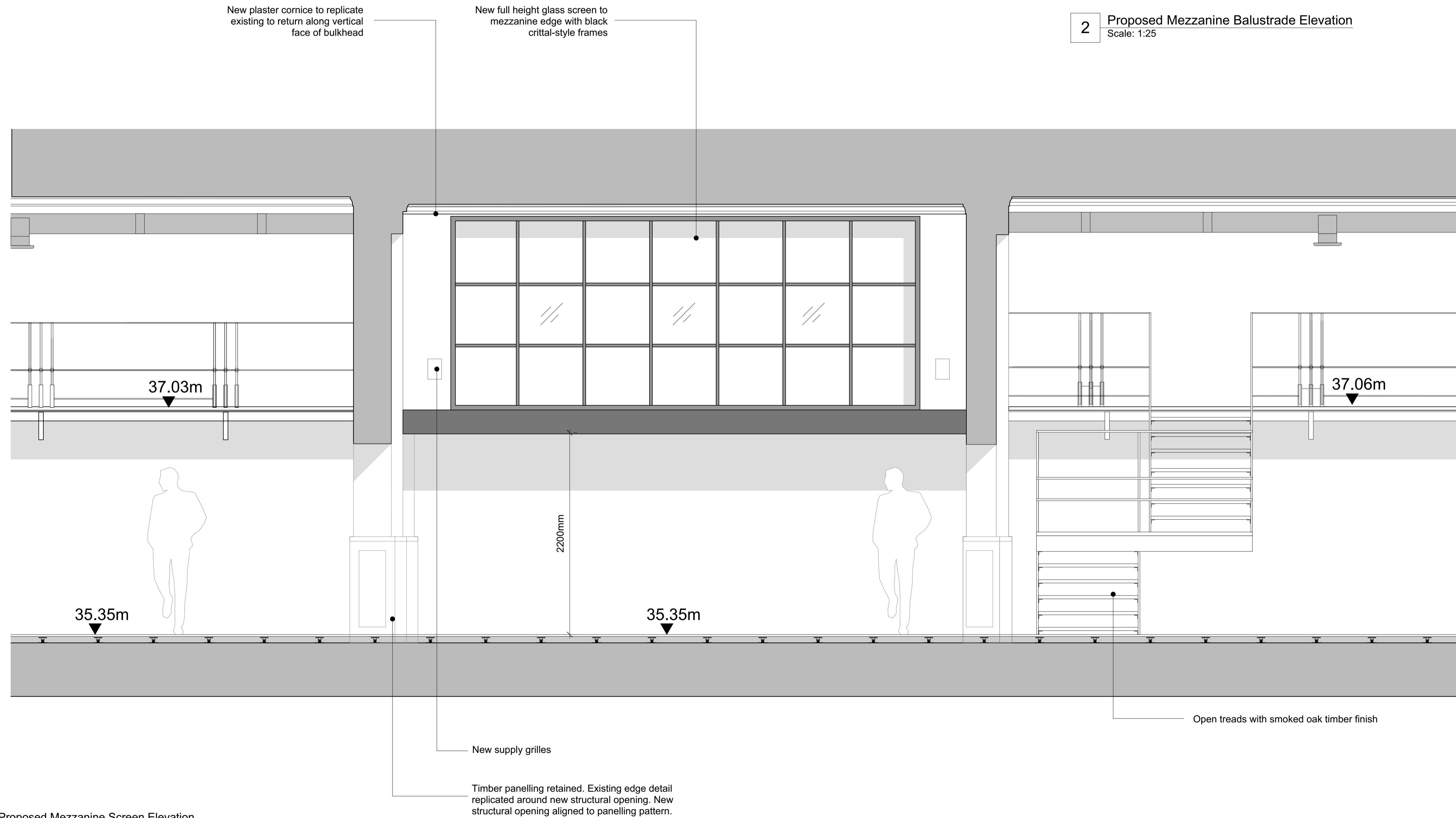
1 Proposed Mezzanine Screen Elevation Scale: 1:25
