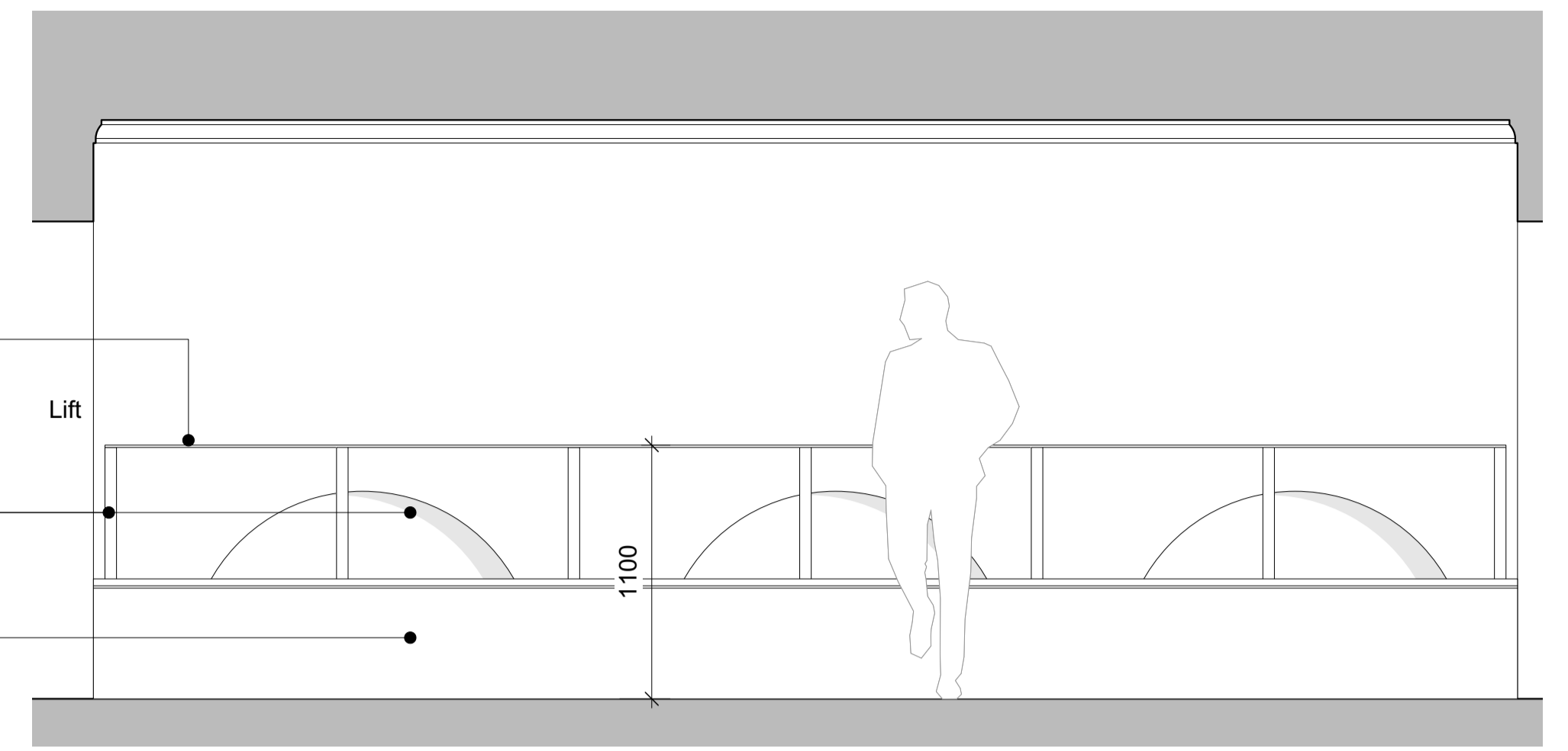
2 Proposed Mezzanine Balustrade Elevation Scale: 1:25
