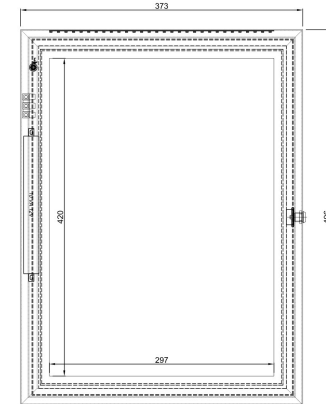
4 Proposed Sign Ø8 elevation Scale: 1:1Ø
