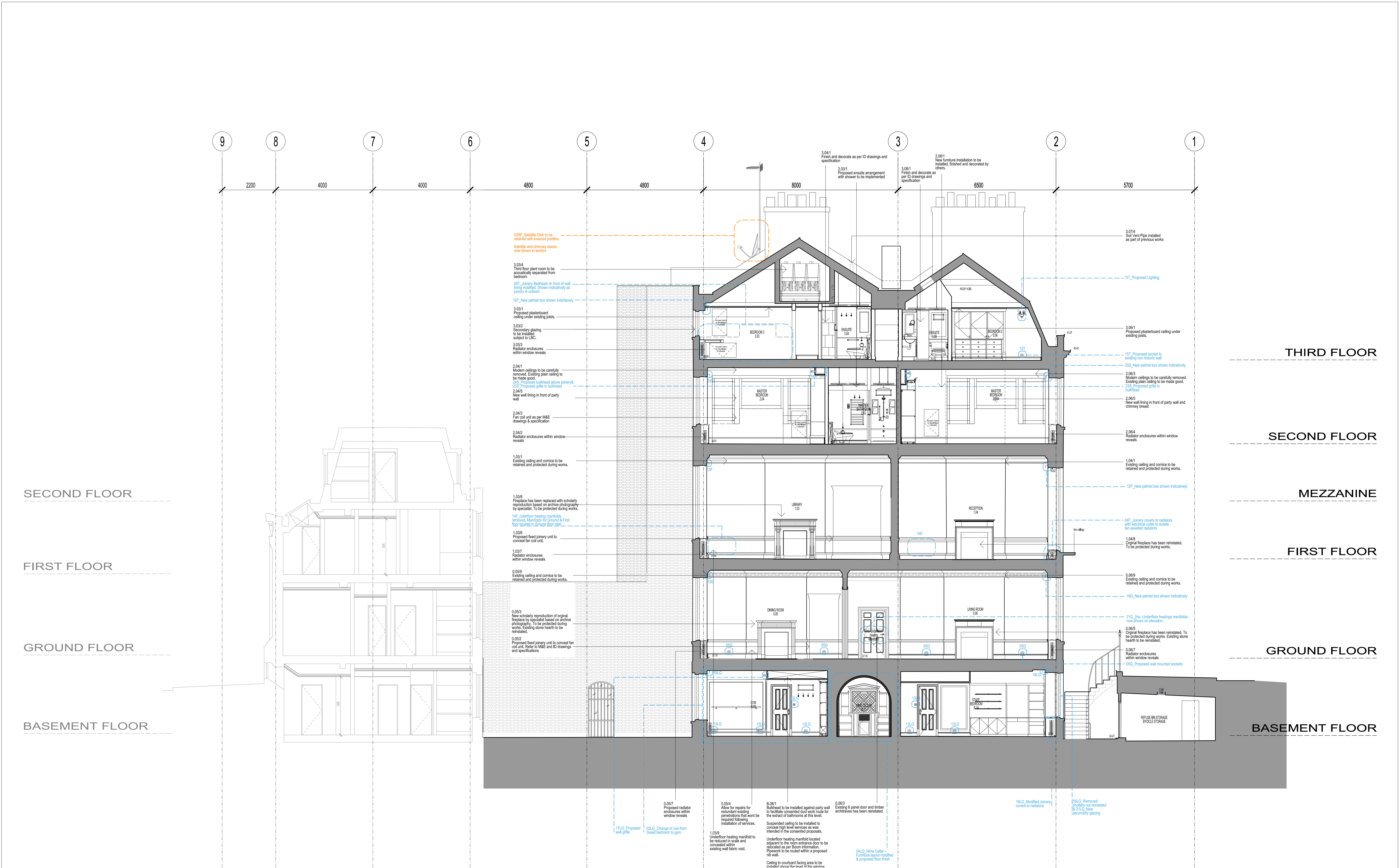
SECTION J - J
