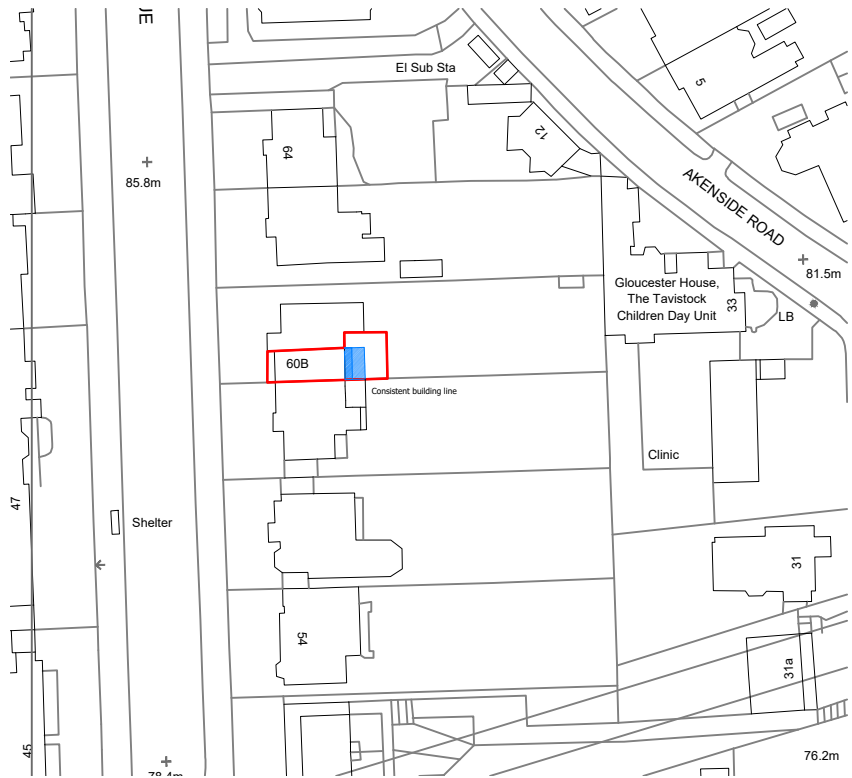
PROPOSED SITE LOCATION PLAN 1.1250
