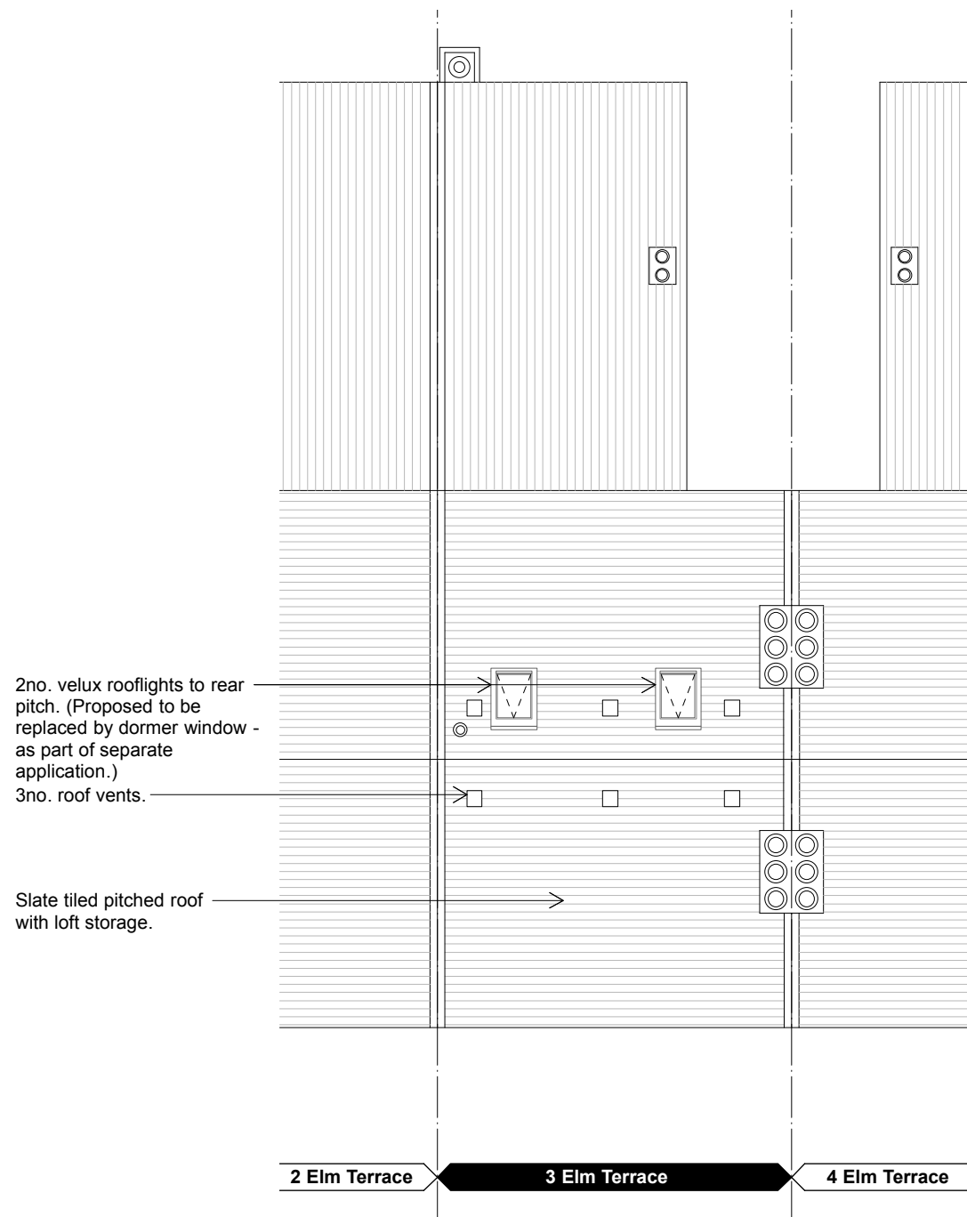
(PL)09_Roof Plan - Existing
