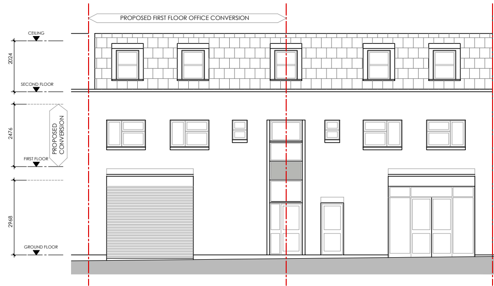
3 FRONT ELEVATION ( NO CHANGES) EXISTING 1:100
