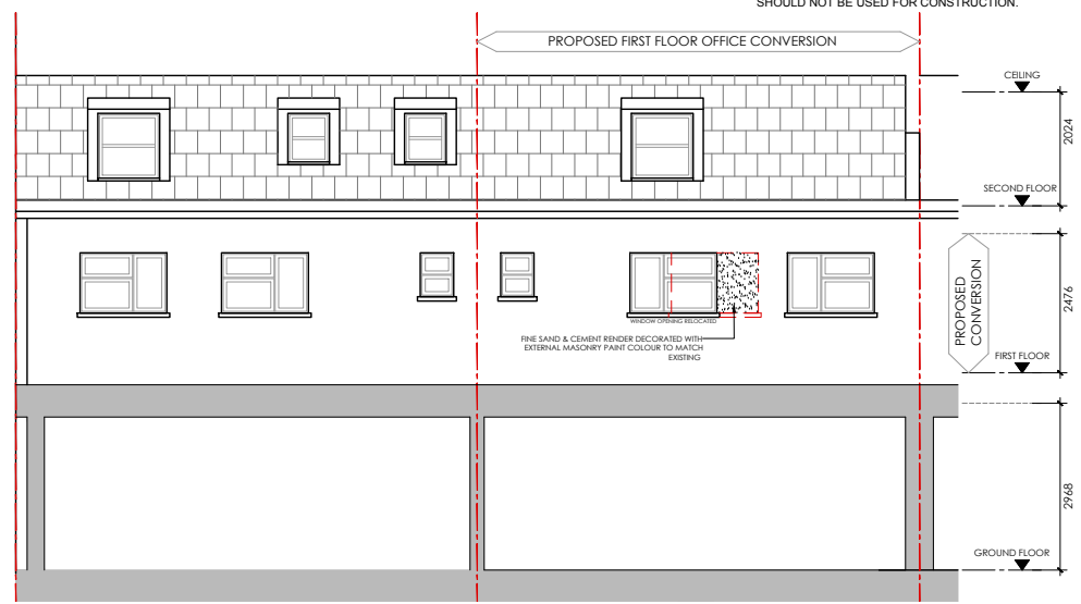
2 REAR ELEVATION PROPOSED 1:100
