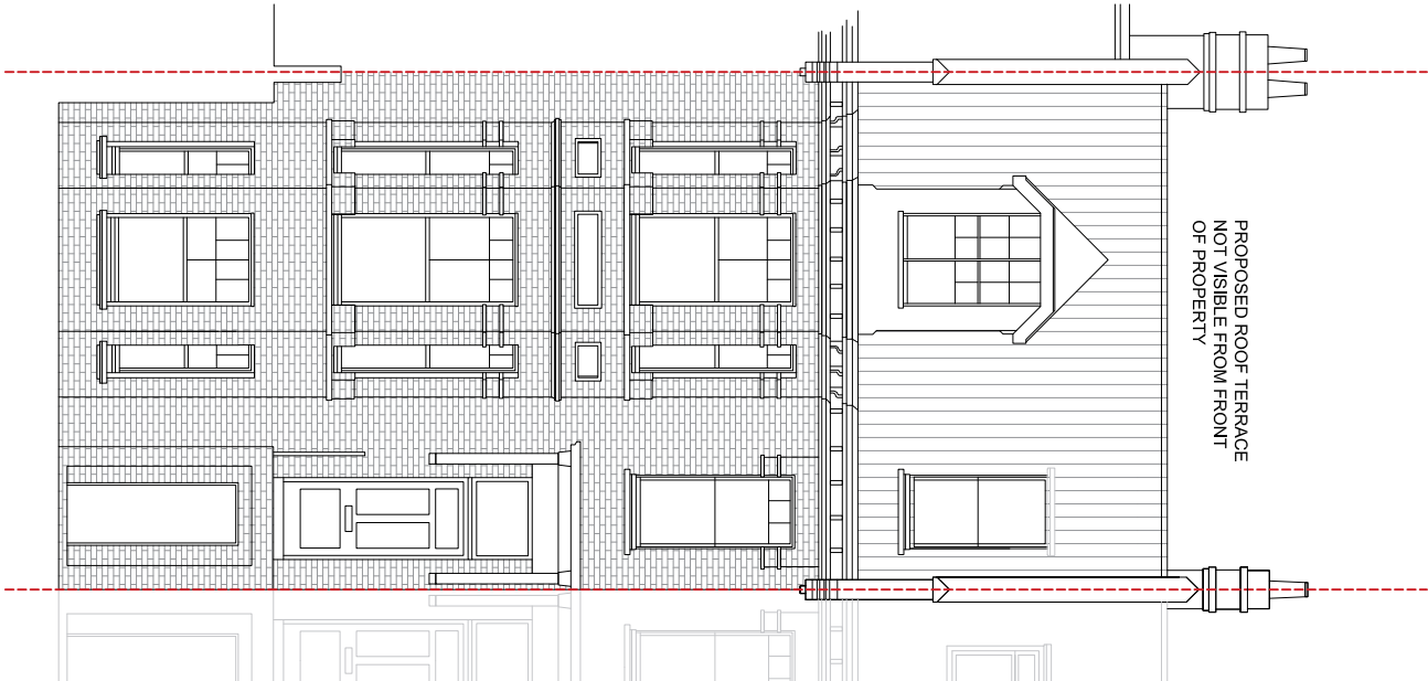
02 Proposed Front Elevation Scale 1:100
