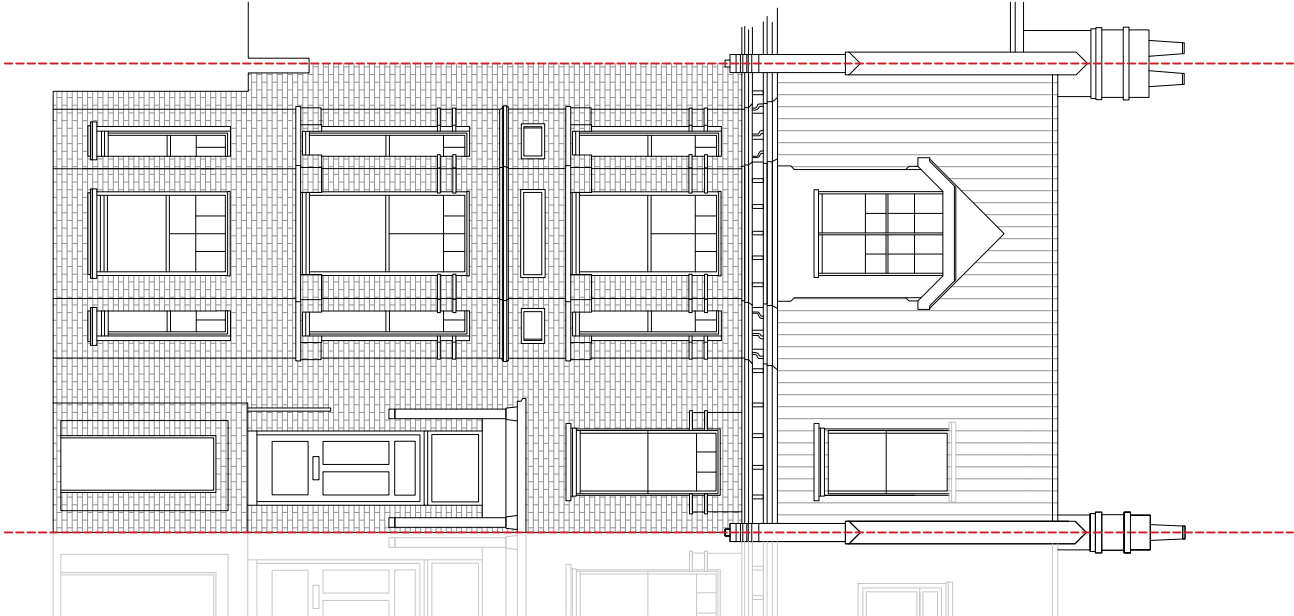
01 Existing Front Elevation Scale 1:100
