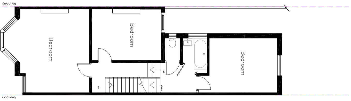
First Floor Plan As Proposed
