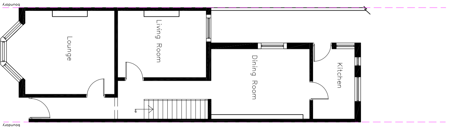
Ground Floor Plan As Proposed
