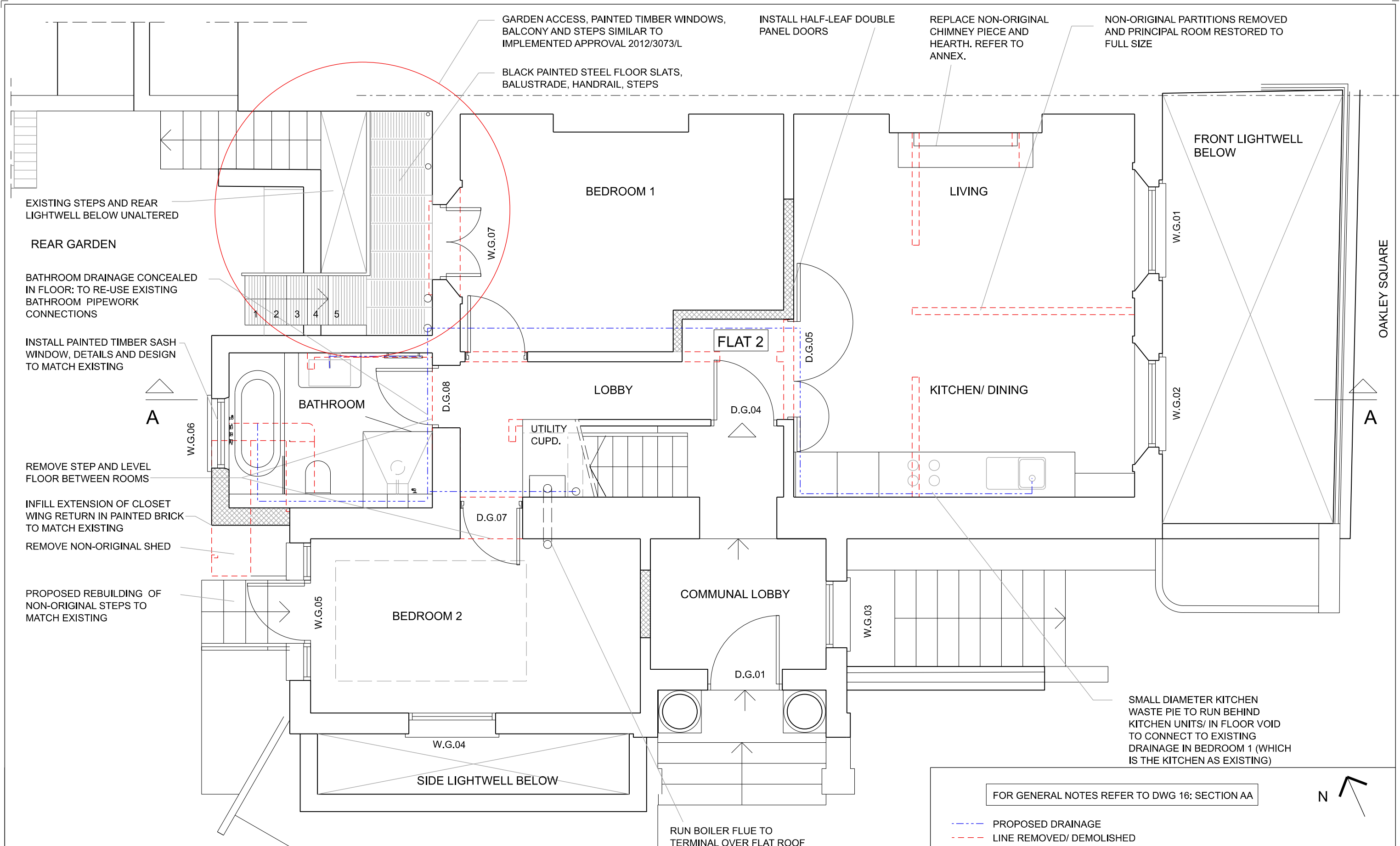
12 A GROUND FLOOR PLAN AS PROPOSED
