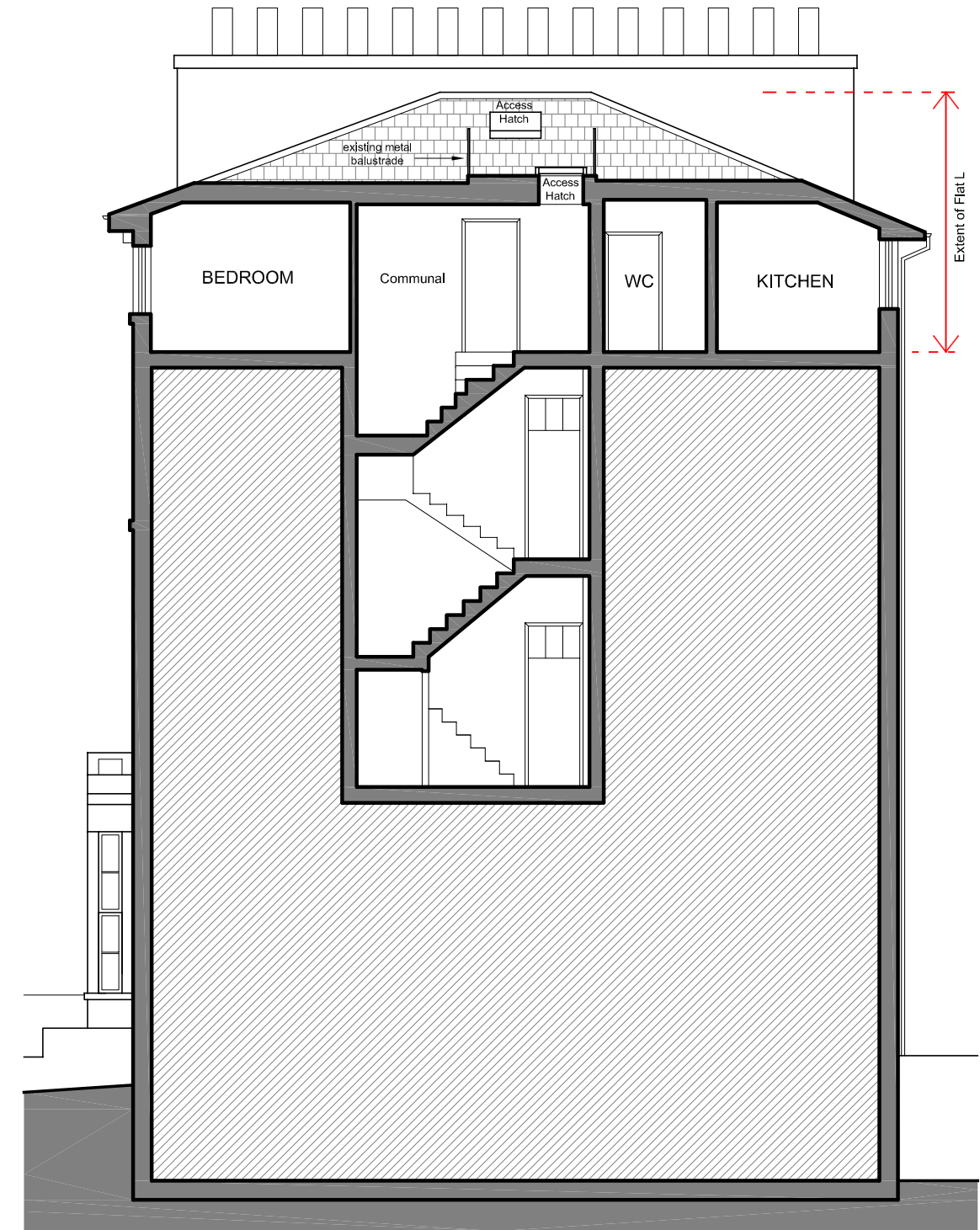
EXISTING - Section A-A Scale 1:100@A3 EX-03
