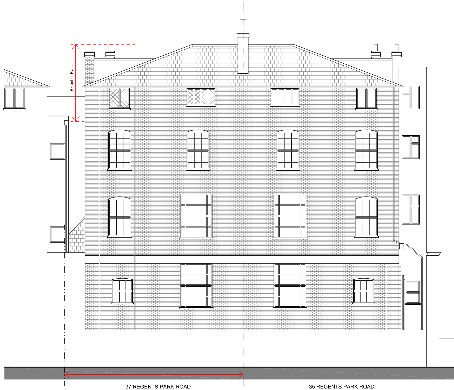
EXISTING - Rear Elevation Scale 1:100@A3 EX-03
