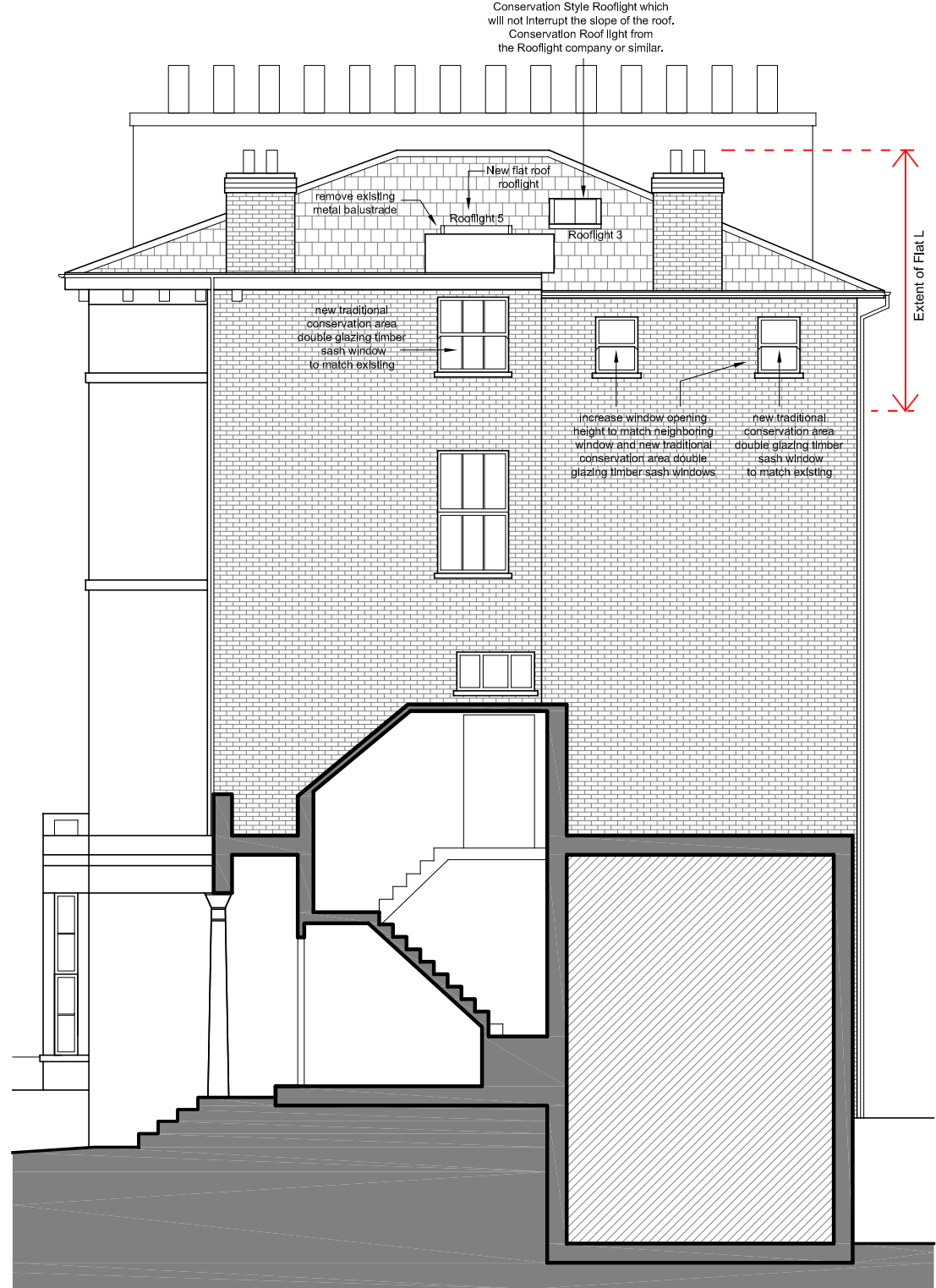
PROPOSED - Side Elevation Scale 1:100@A3 PA-02
